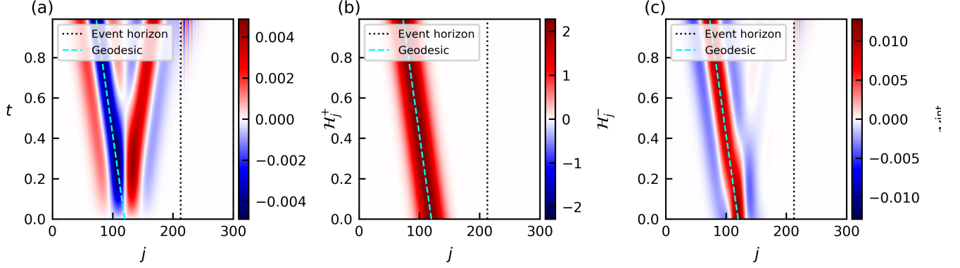
FIG. 5. Wave-packet dynamics in the black-hole geometry for p = 1 for an initially prepared a^- wave packet outside the horizon. The parameters and horizon position are the same as in Fig. 4, except that the packet is initialized at j_{\text{ini}} = 120 . Panels (a)–(c) show the vacuum-subtracted contributions \delta\mathcal{E}_{j,+}(t) , \delta\mathcal{E}_{j,-}(t) , and \delta\mathcal{E}_{j,\text{int}}^{(-)}(t) , respectively. Black dotted lines indicate the horizon, and cyan dashed curves show the corresponding continuum null trajectories obtained from Eq. (24).
