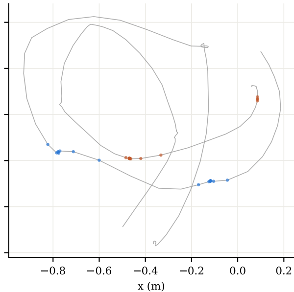
Ours (full)
