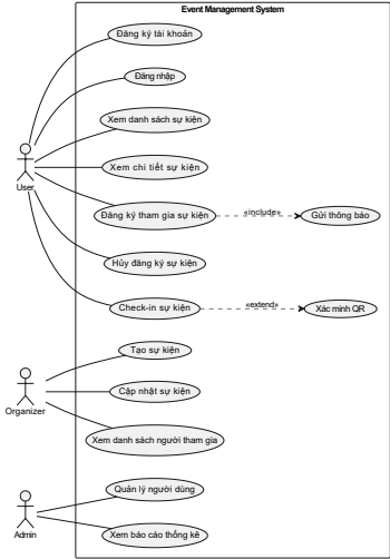
Use Case Diagram
