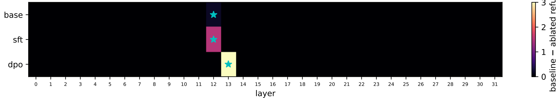
Causal refusal strength across the alignment pipeline
