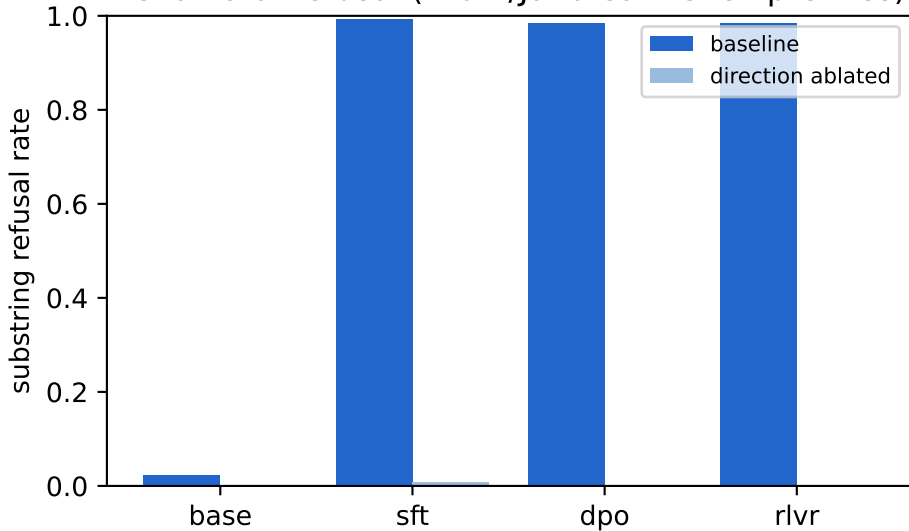
Behavioral refusal (Arditi/JailbreakBench prefixes)
