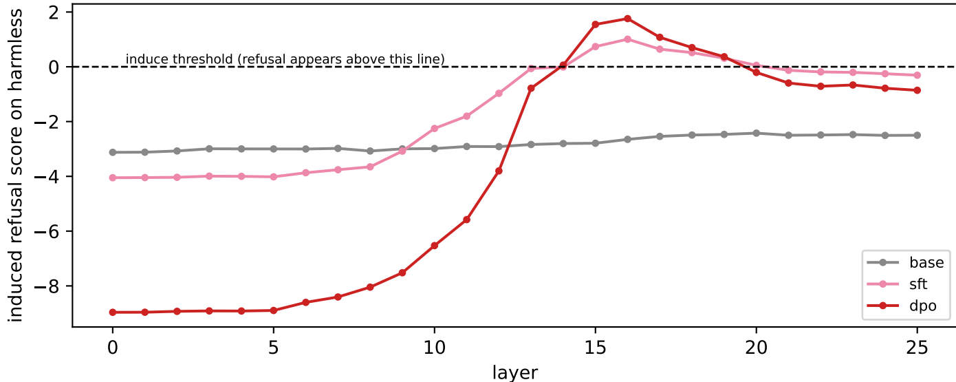
Can refusal be STEERED IN? (direction added to harmless prompts)
