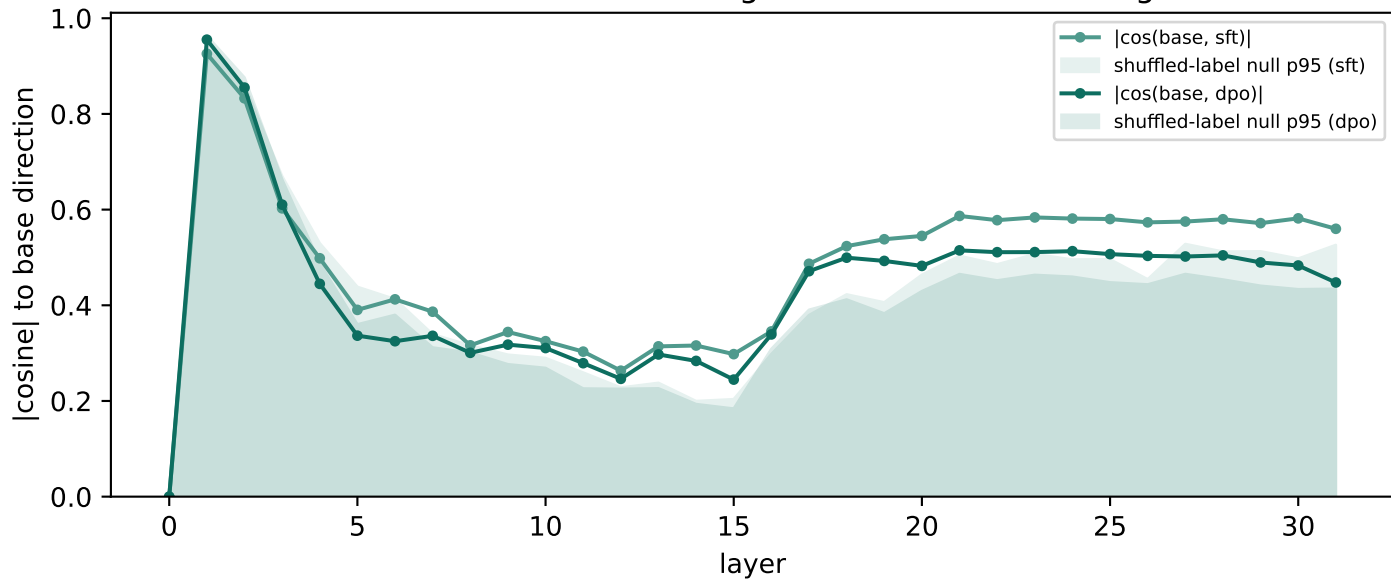
Is it the SAME axis the aligned model refuses along?
