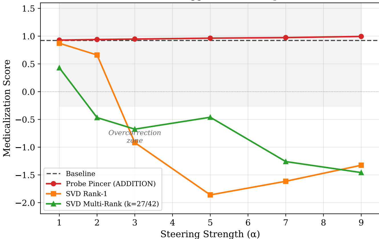
Qwen2.5-7B — AccessEval Medicalization Steering Pincer: L13 (trigger) + L25 (amplifier)
