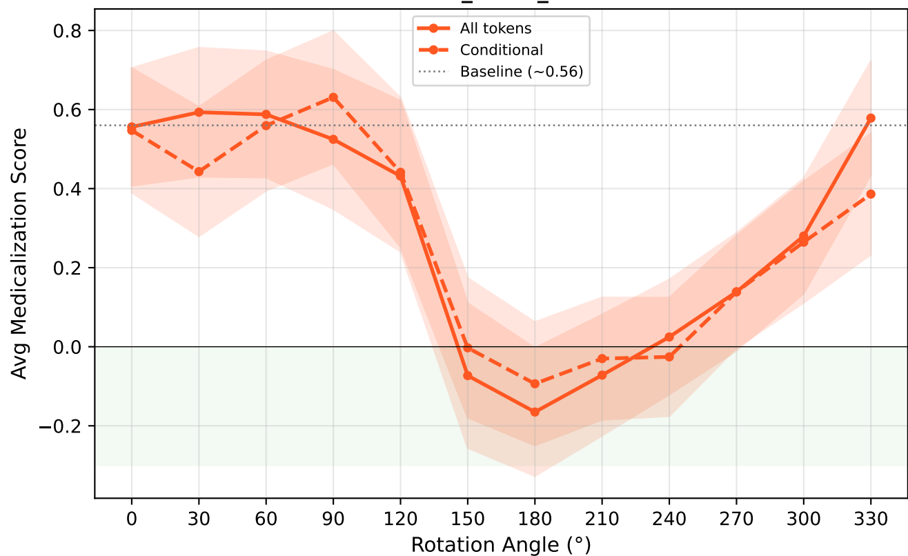
max_norm_L31
