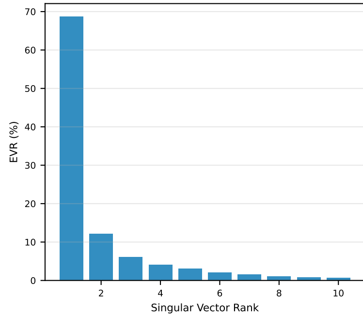
Llama Target A L15 (amplifier) top-1=67.9%, k@80%=1
