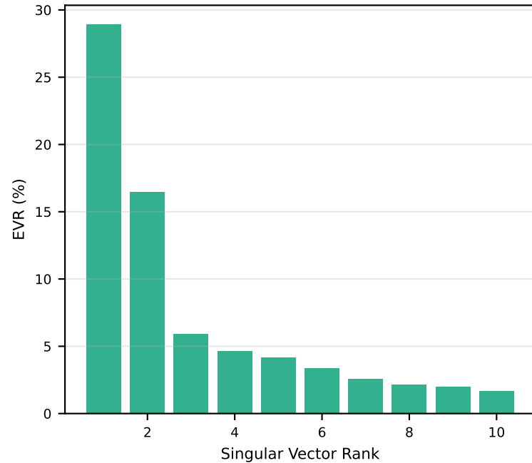
Mistral Target B L31 (amplifier) top-1=28.9%, k@80%=17
