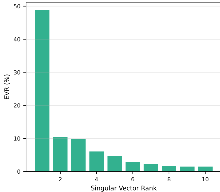
Mistral Target A L31 (amplifier) top-1=48.8%, k@80%=6
