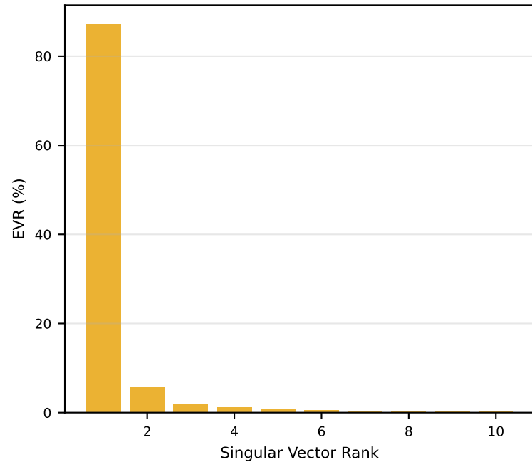
Qwen Target A L26 (amplifier) top-1=87.1%, k@80%=1
