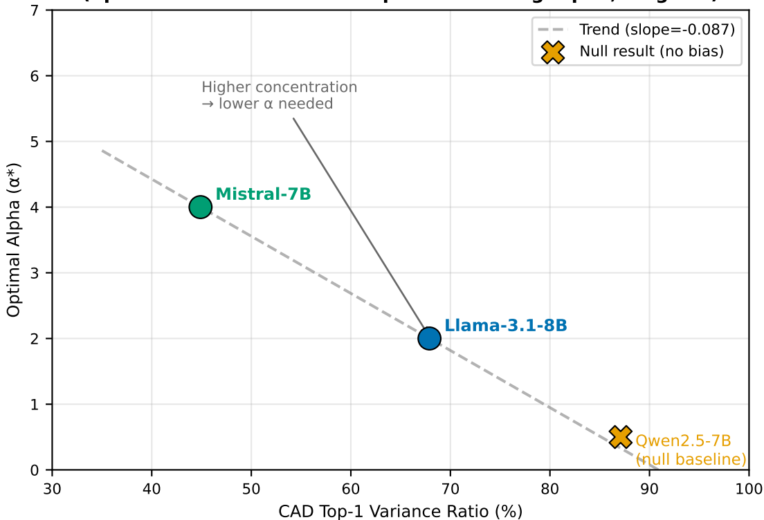
Figure 4: CAD Alpha Scaling Law (Spectral Concentration vs Optimal Steering Alpha, Target A)
