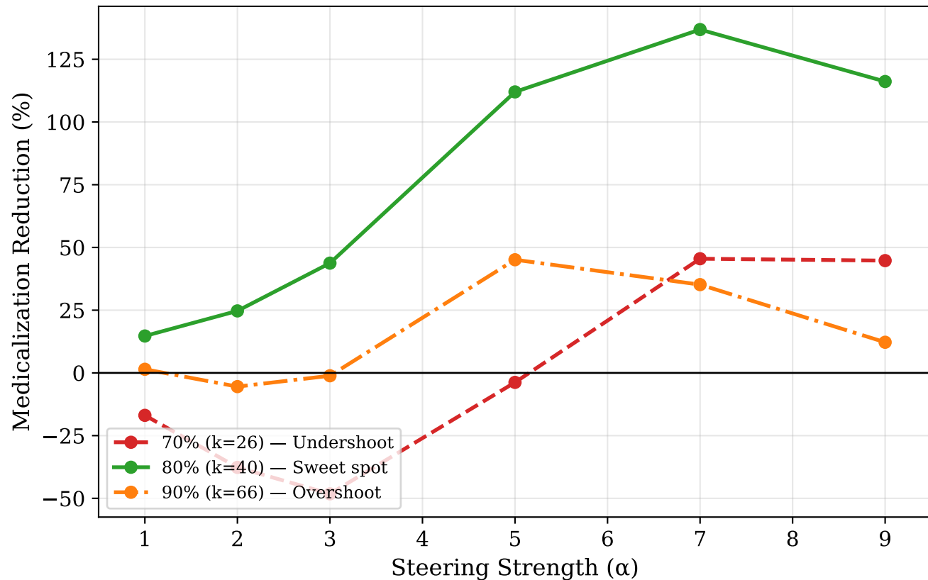
Alpha Sweep by Threshold (Phase transition between 70% and 80%)
