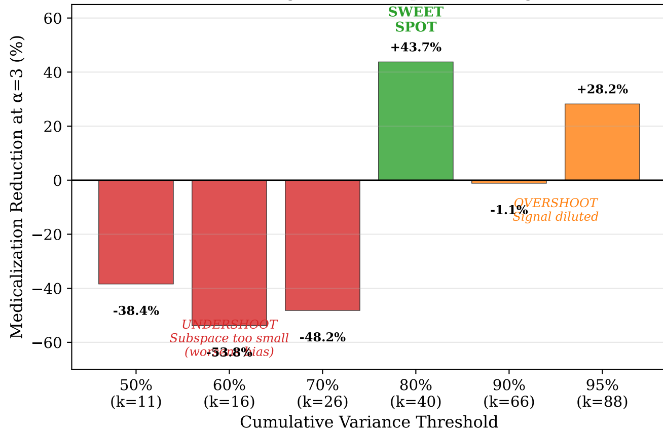
Three Regimes of Subspace Steering
