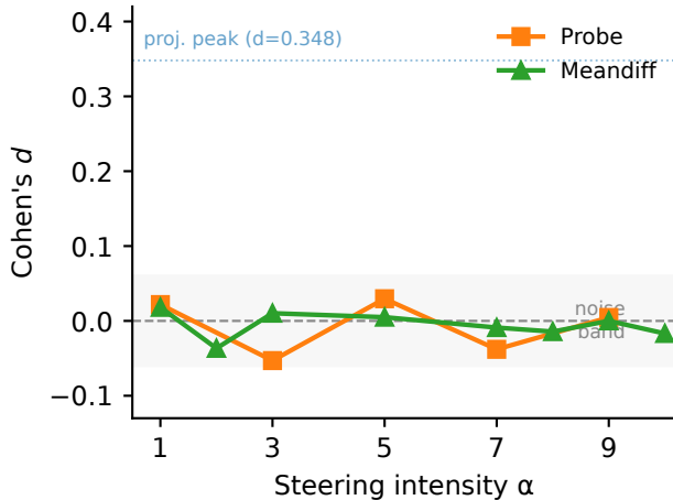
(B) Probe & Meandiff (both NS)
