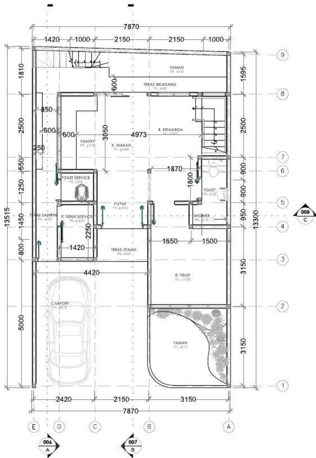
DENAH LANTAI DASAR
