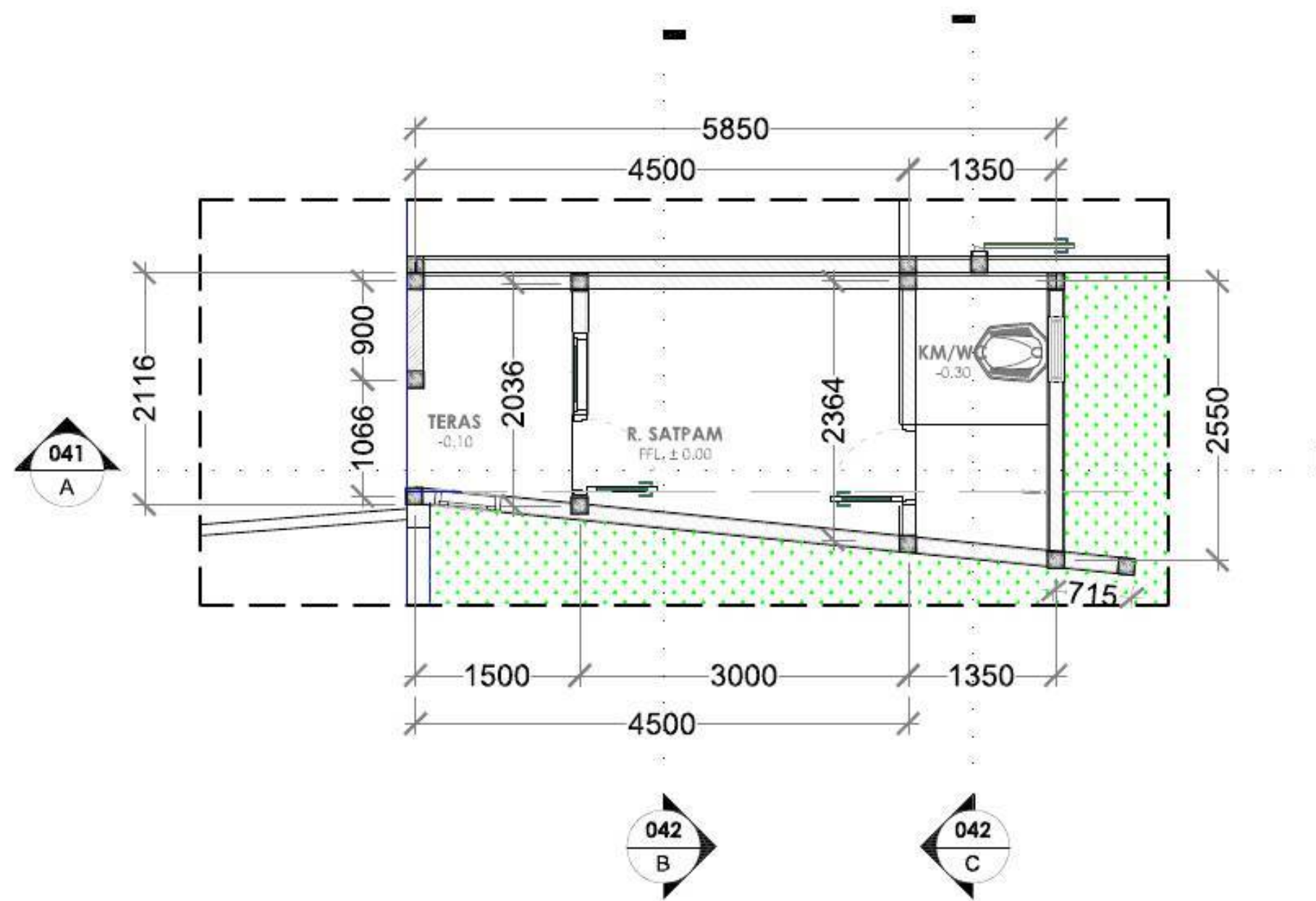
DENAH RG. SATPAM SKALA 1: 50
