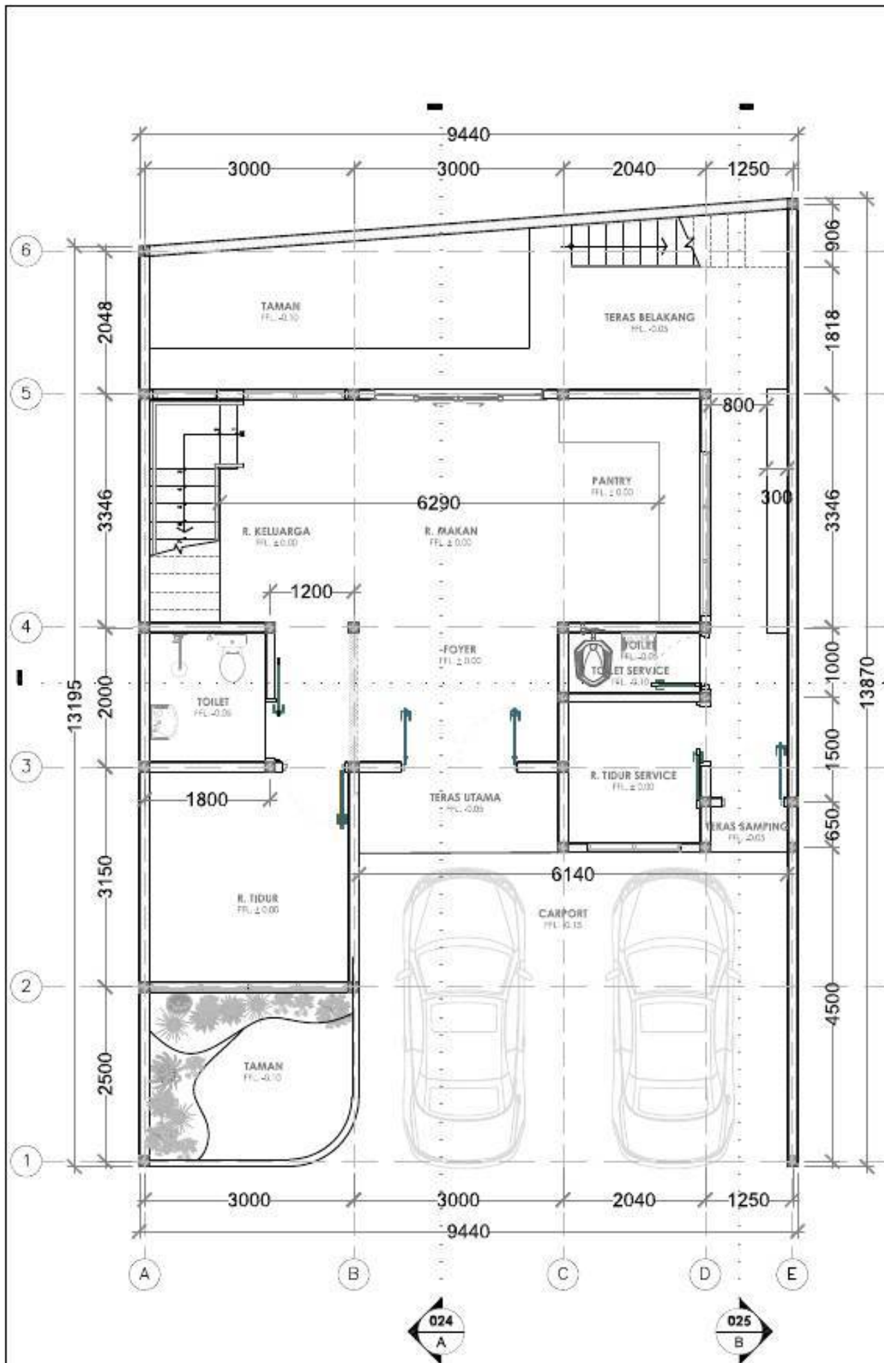
DENAH LANTAI DASAR SKALA 1: 75
