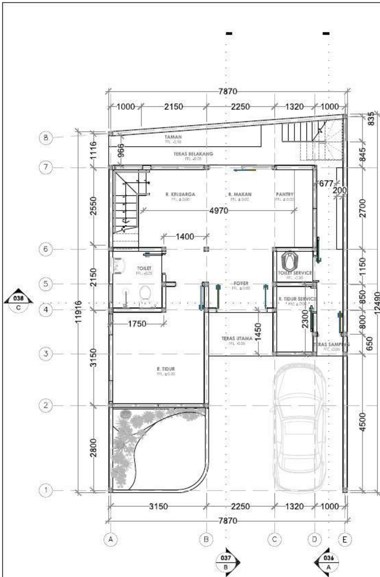
DENAH LANTAI DASAR SKALA 1: 75
