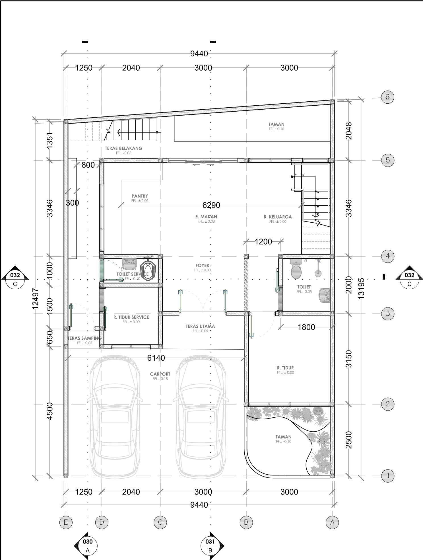
DENAH LANTAI DASAR SKALA 1: 75
