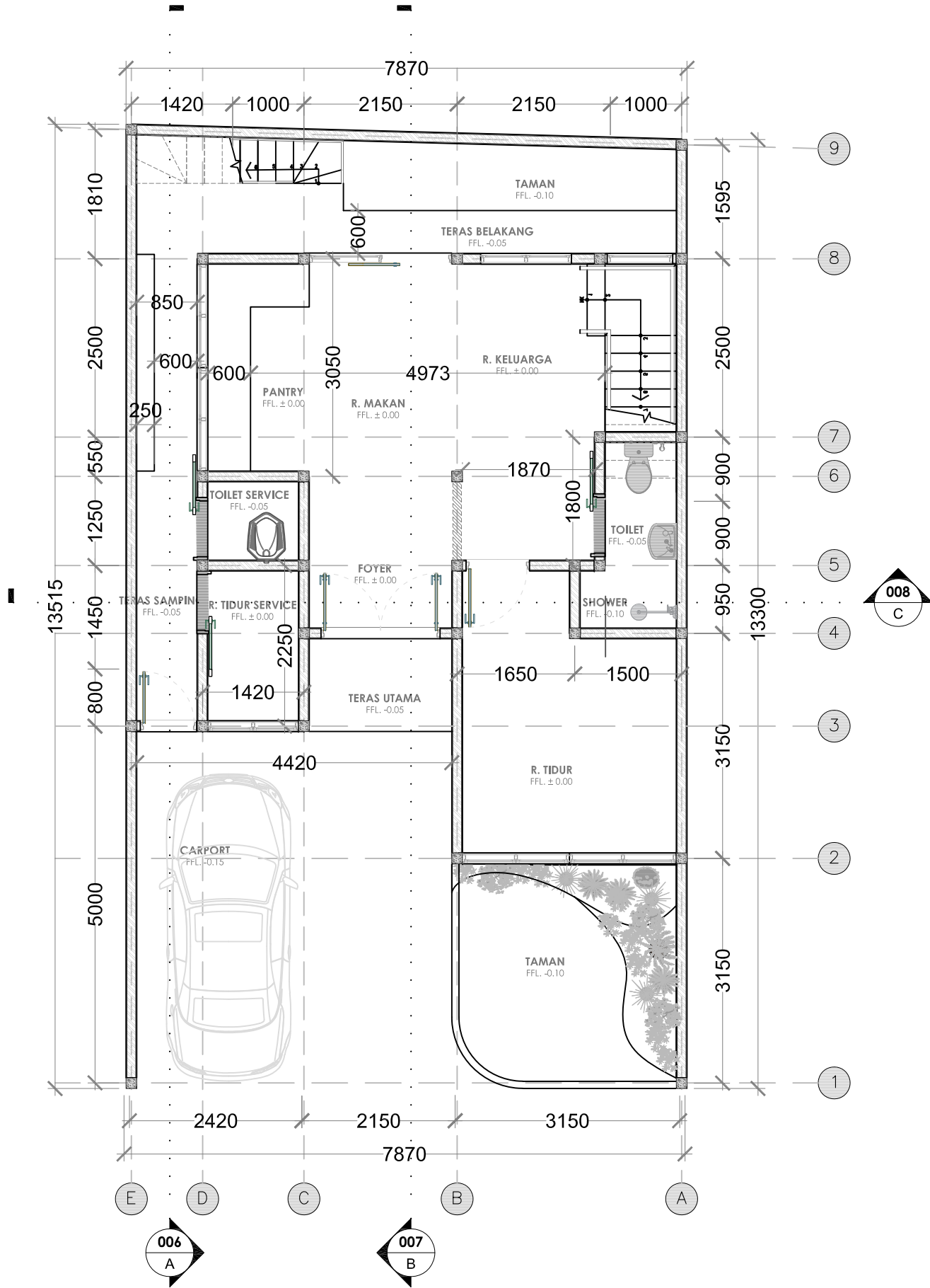
DENAH LANTAI DASAR SKALA 1: 75
