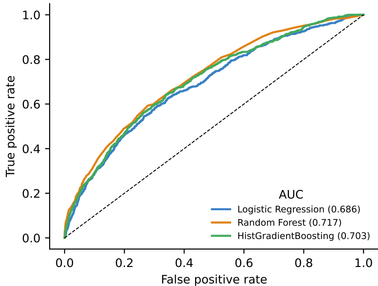
(a) ROC curves
