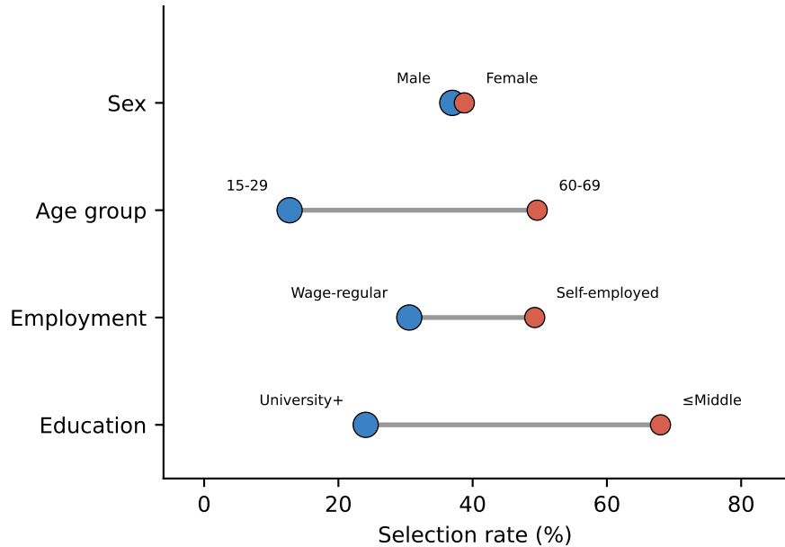
(b) Selection-rate disparity by group
