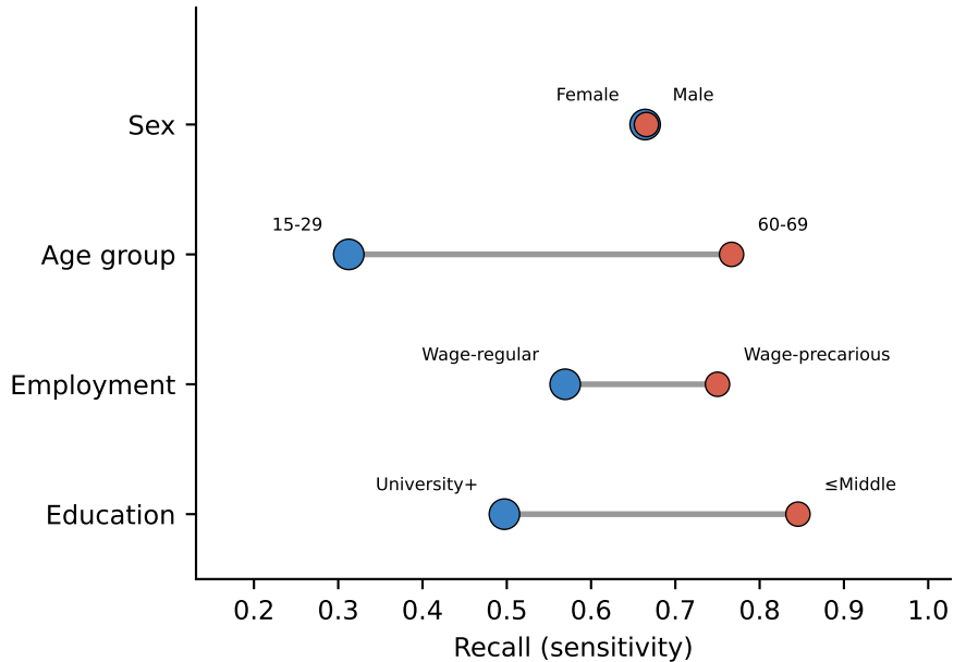
(a) Recall (TPR) disparity by group
