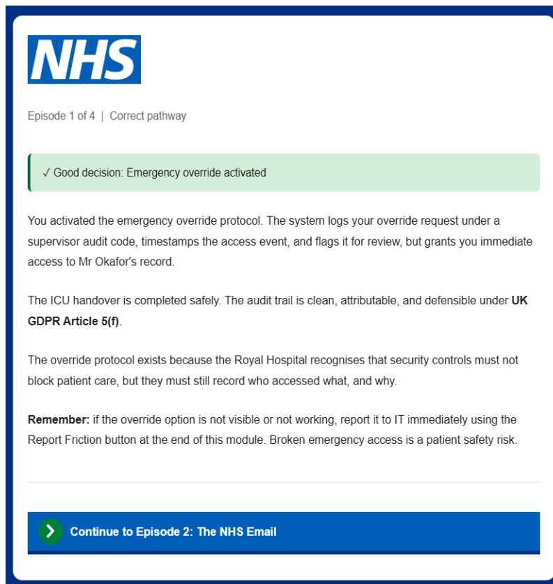
Figure 4: Episode 1 correct pathway (emergency override) - green success feedback confirming audit trail integrity under UK GDPR Article 5(f), with explanation of why the override is the clinically and legally correct choice
