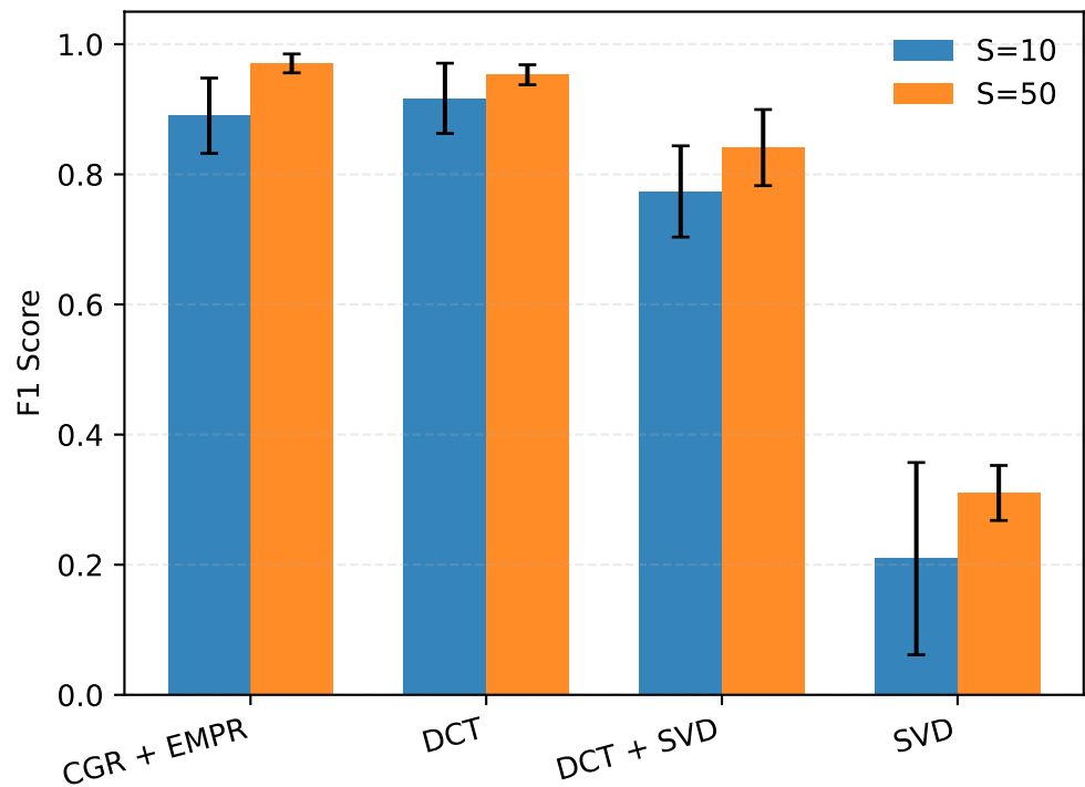
Imbalanced 1:4 (S=10 and S=50)
