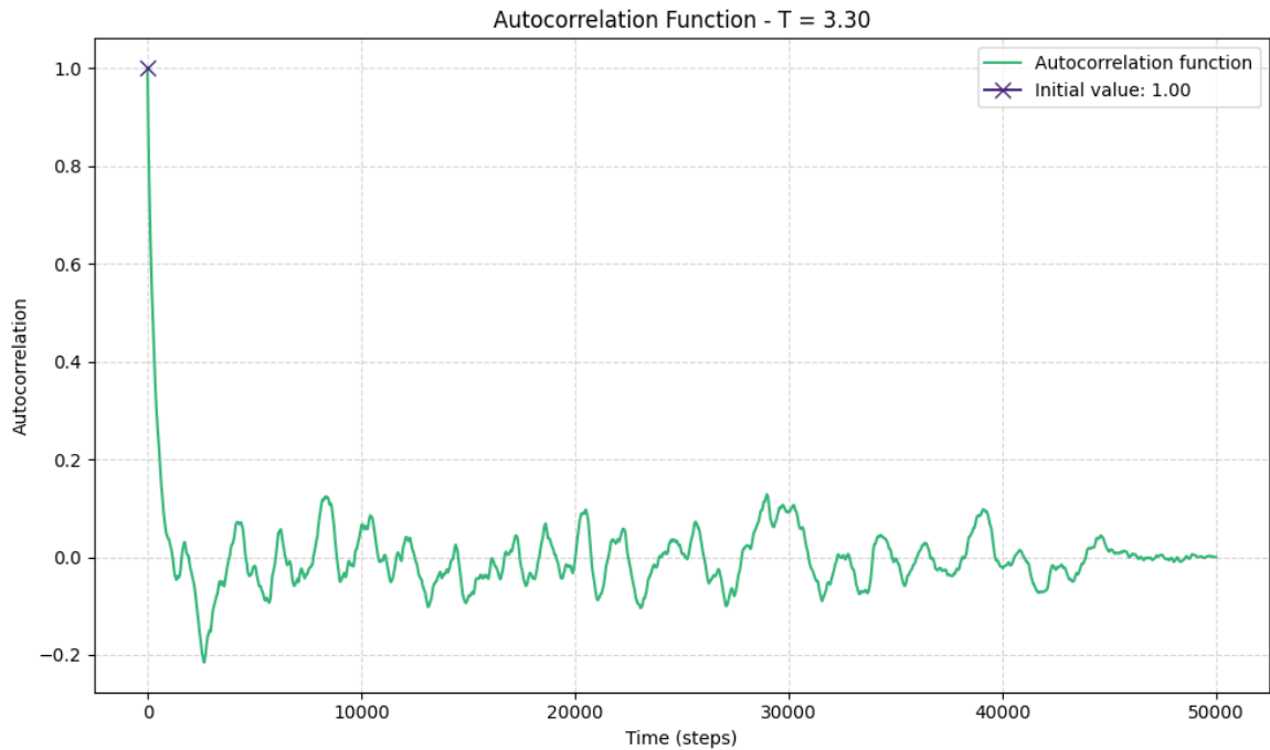
Figure 2.3: Example of autocorrelation function (of the energy) for a Markov Chain.
