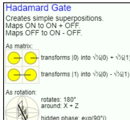
Hadamard Gate transformation
