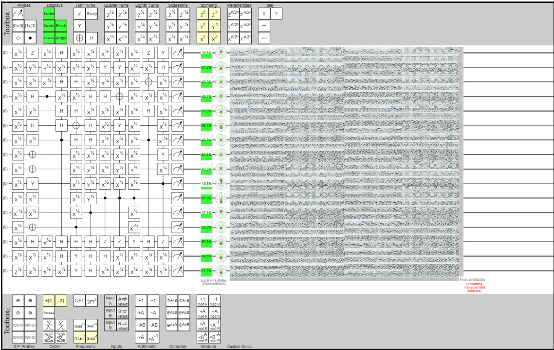
Quantum score with Quirk
