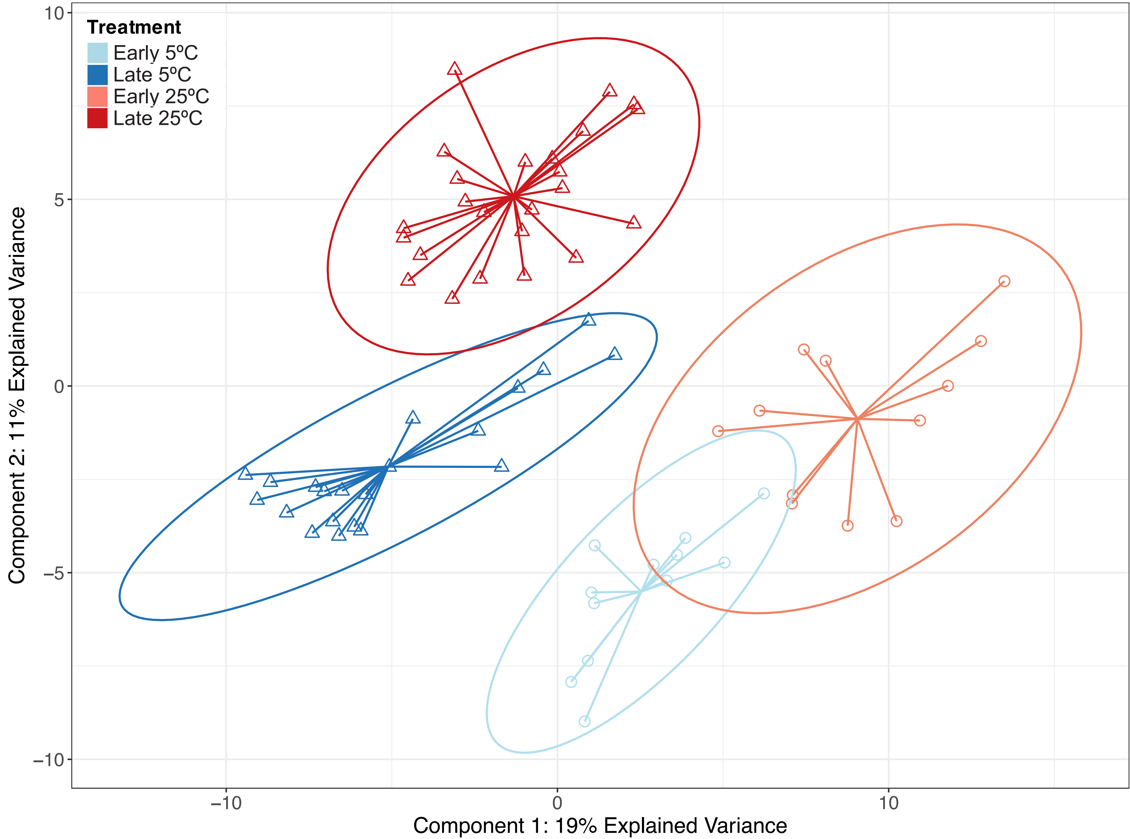
A. Metabolomics PLS-DA by Temperature and Timepoint
