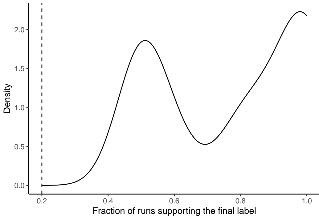
Consensus support density — input_example
