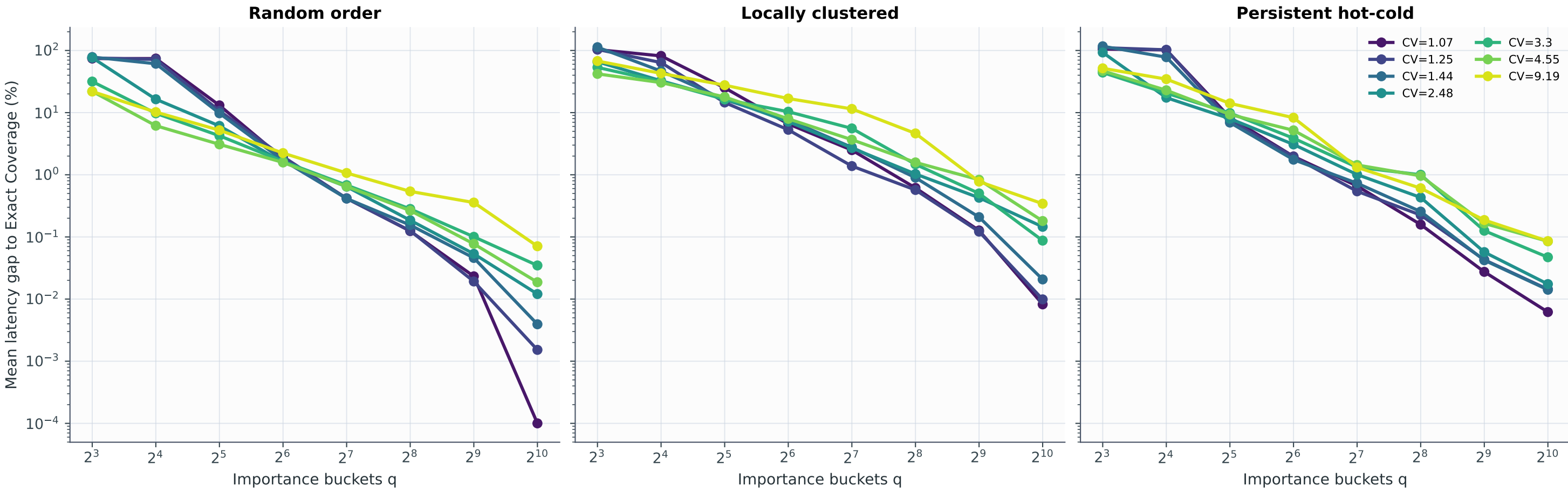
Quantized Pareto accuracy as q increases
