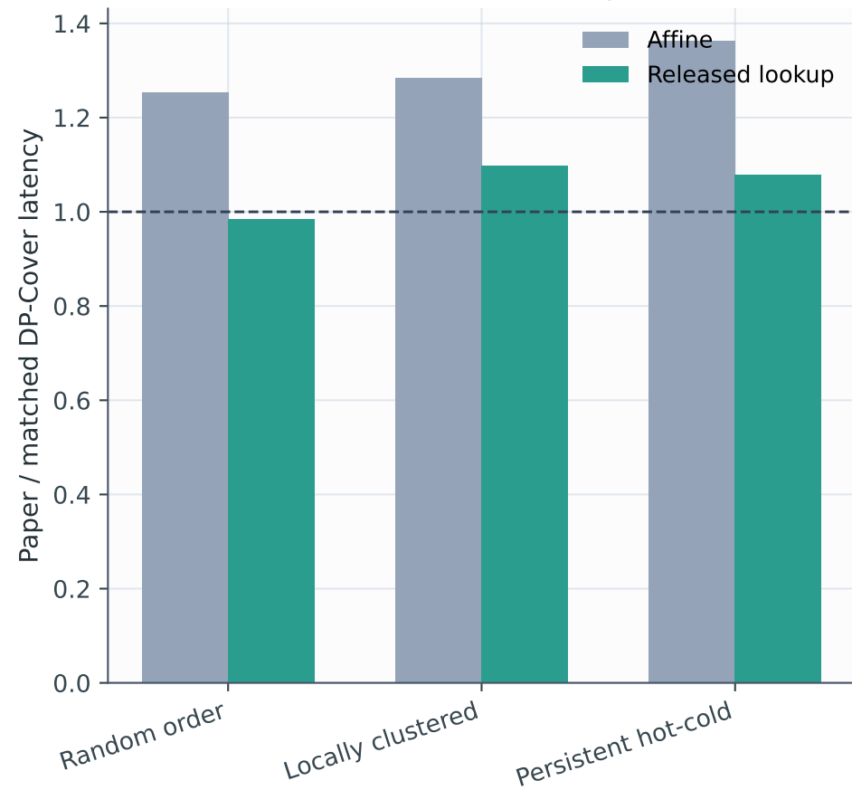
A. Apparent Paper gap
