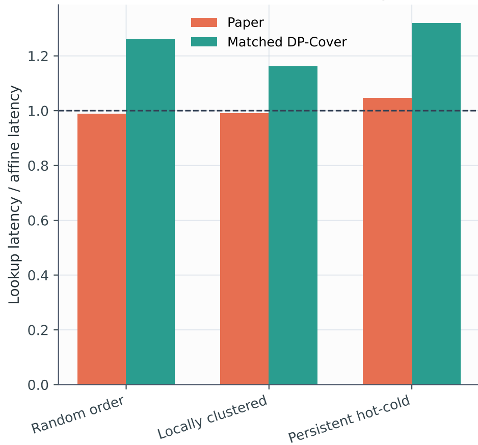
B. Unequal model rescaling
