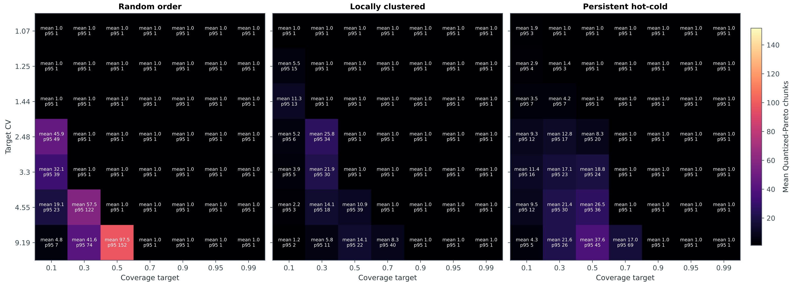
Quantized Pareto q=1024 chunks: N=18944, row=7 KiB
