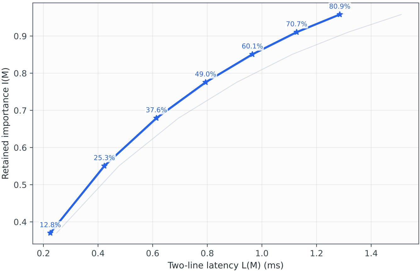
Exact global coverage
