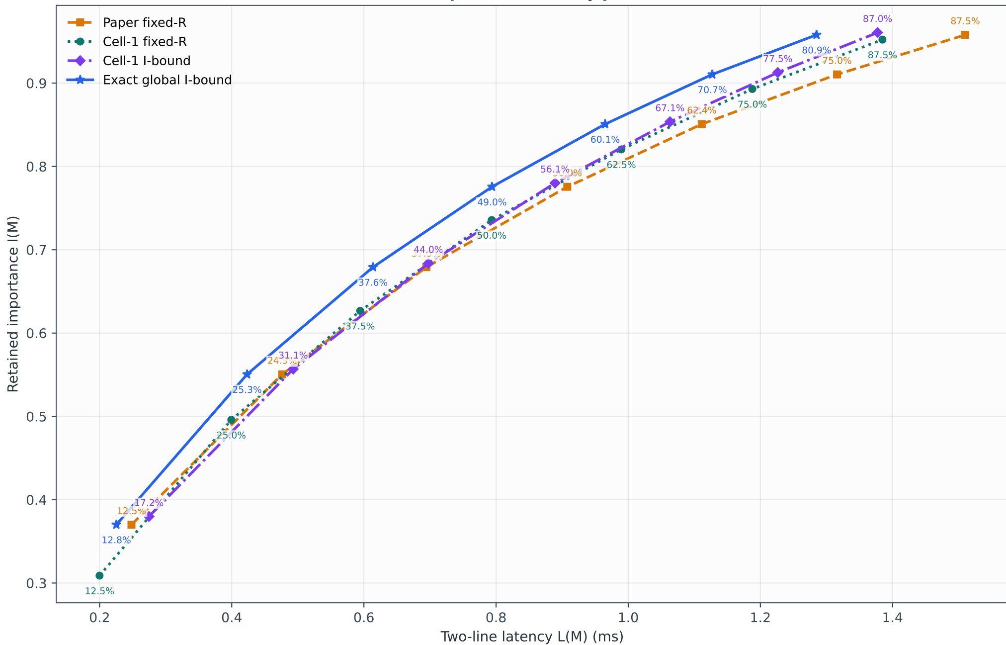
One theoretical importance-latency plane (macro mean)
