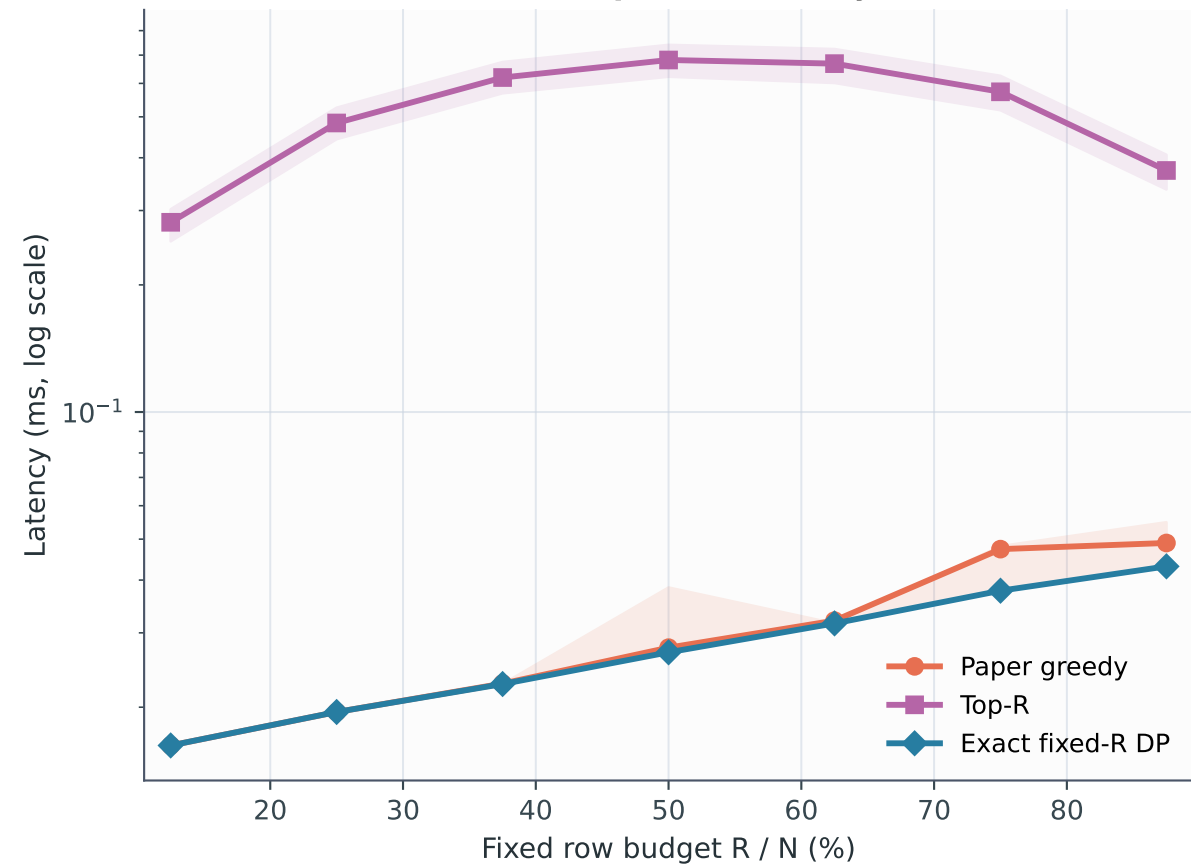
B. Lookup-table latency
