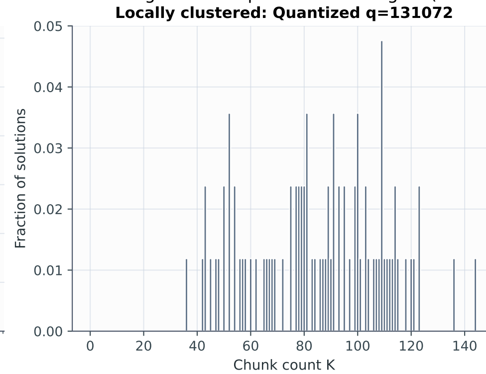
Chunk-count histograms at Paper-matched targets (N=18,944)
