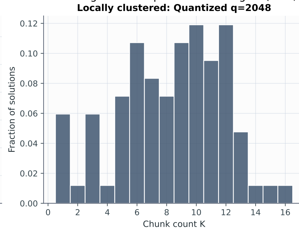
Chunk-count histograms at Paper-matched targets (N=4,864)
