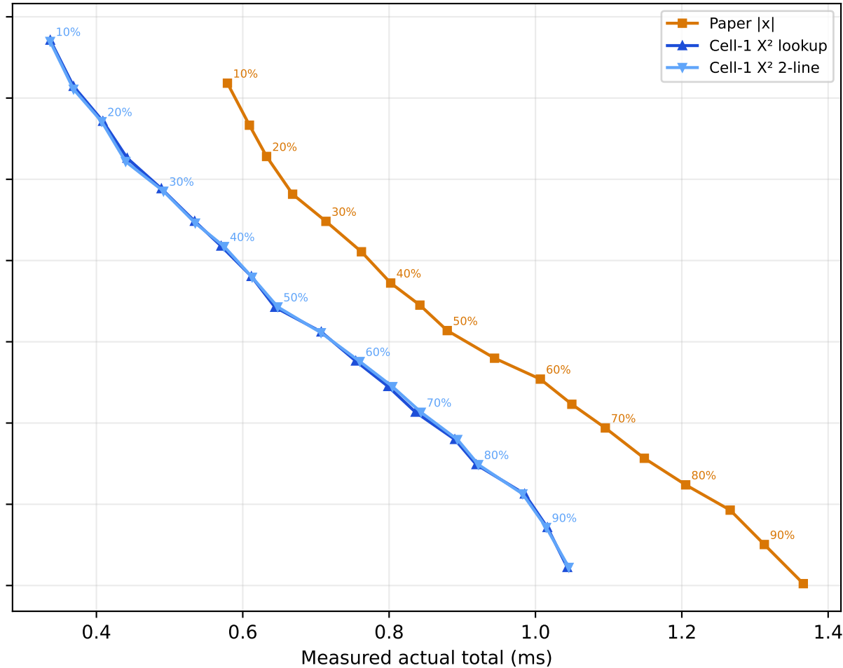
X 2 score
