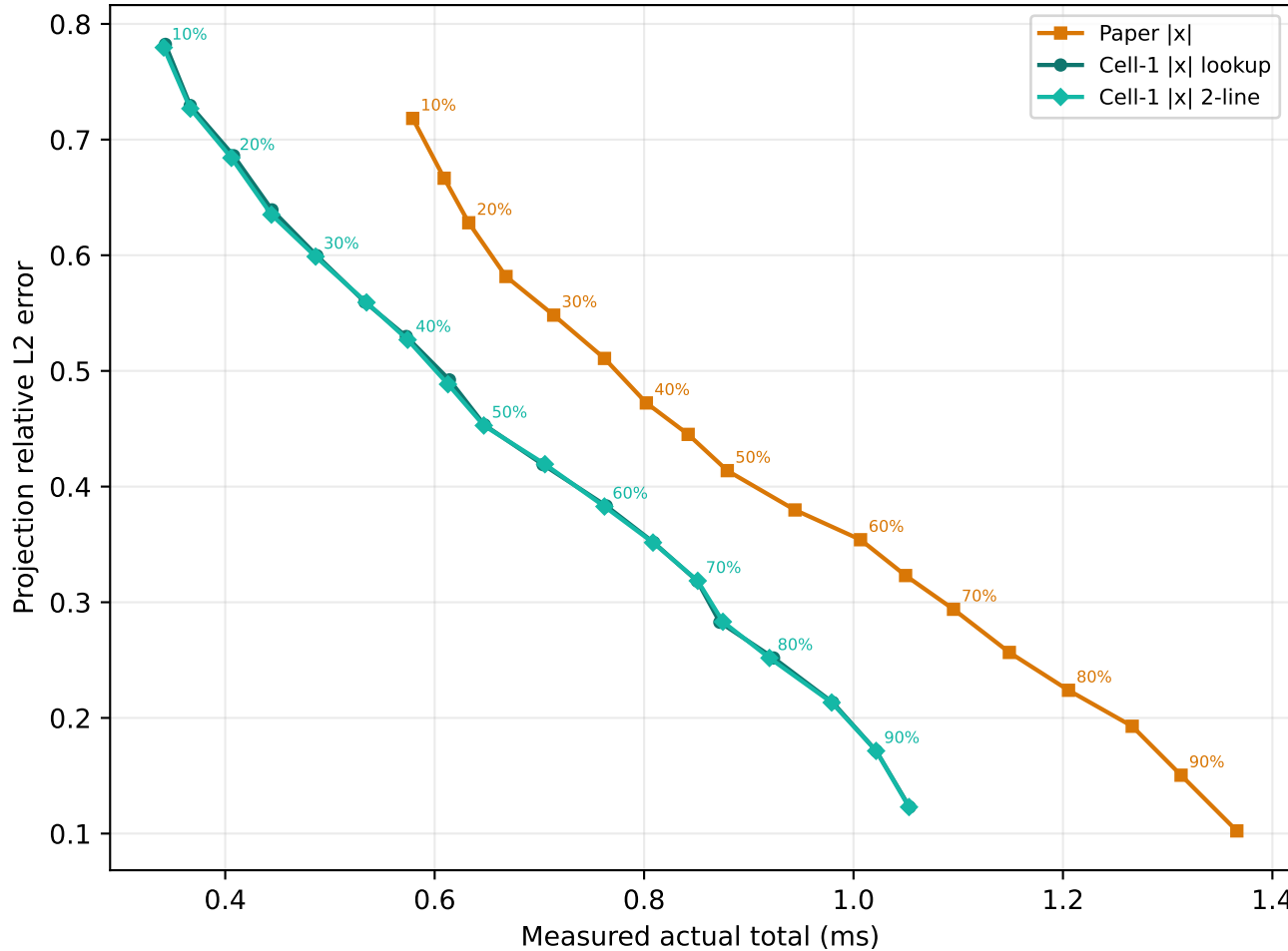
ABS score
