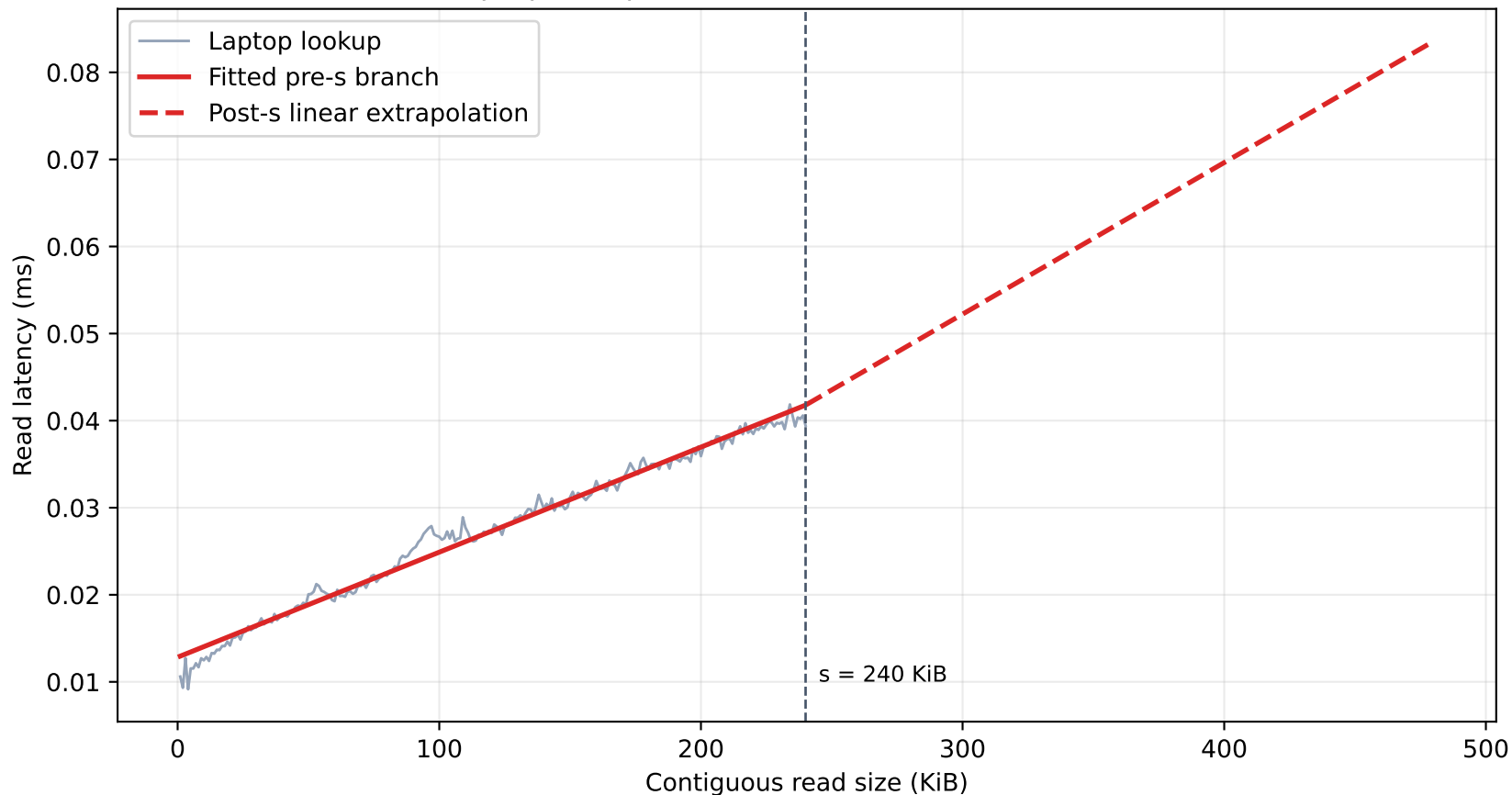
Laptop SSD profile fit ( R^2=0.9854 , MAPE=3.29%)
