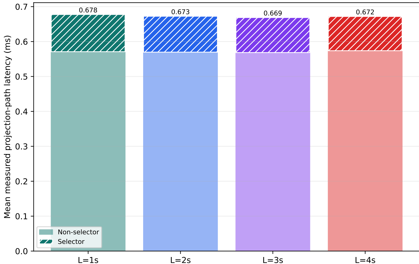
Tile-length latency decomposition
