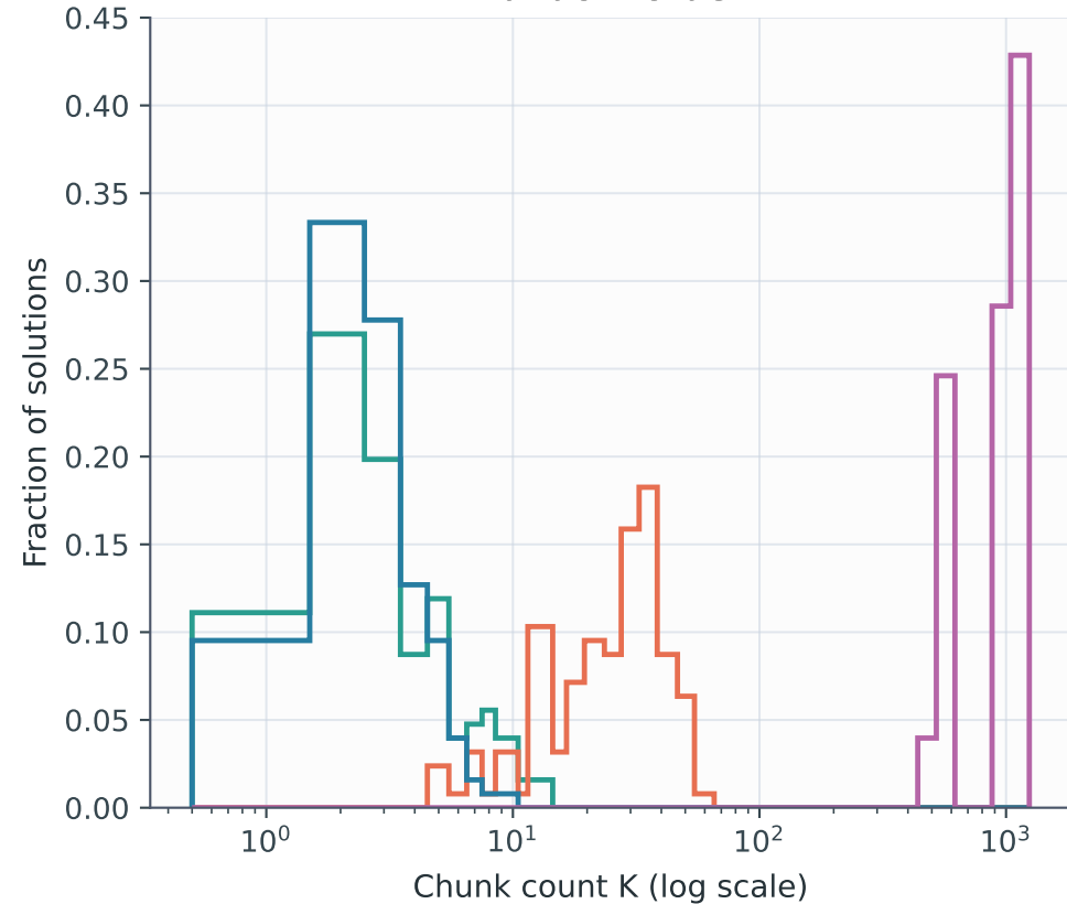
Random order
