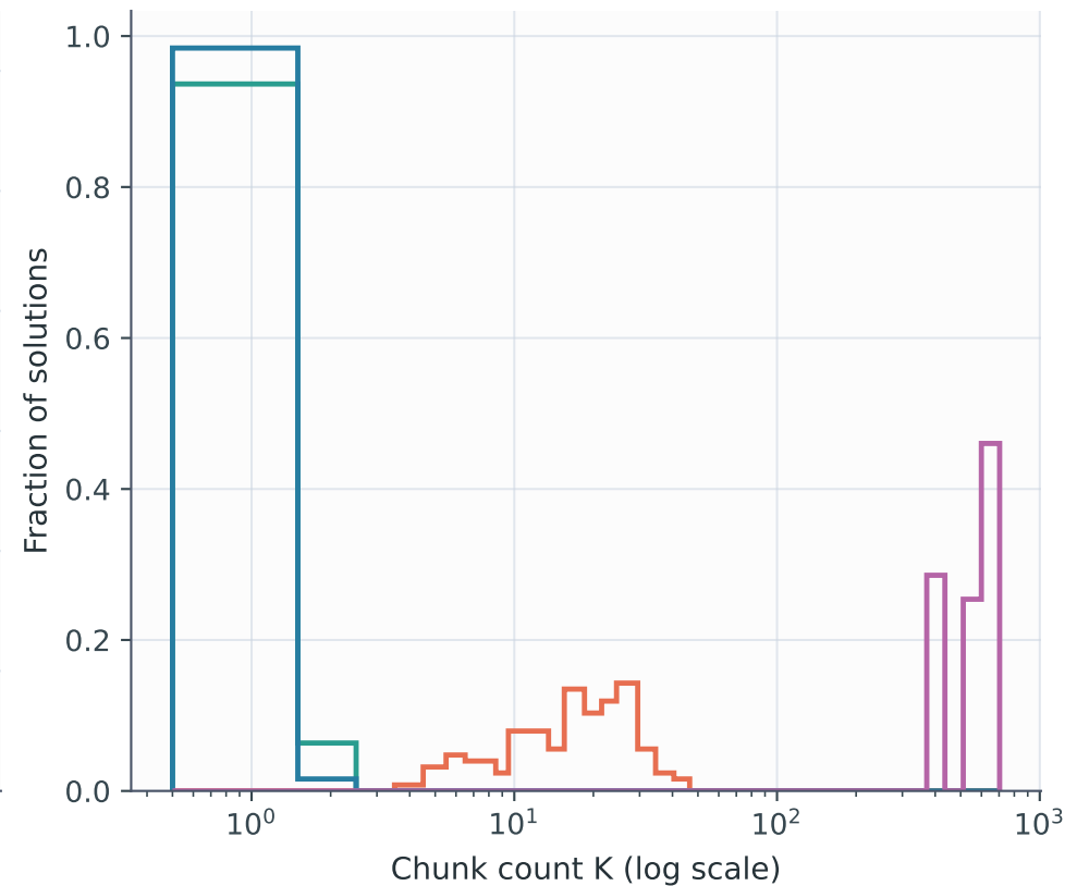
Persistent hot-cold
