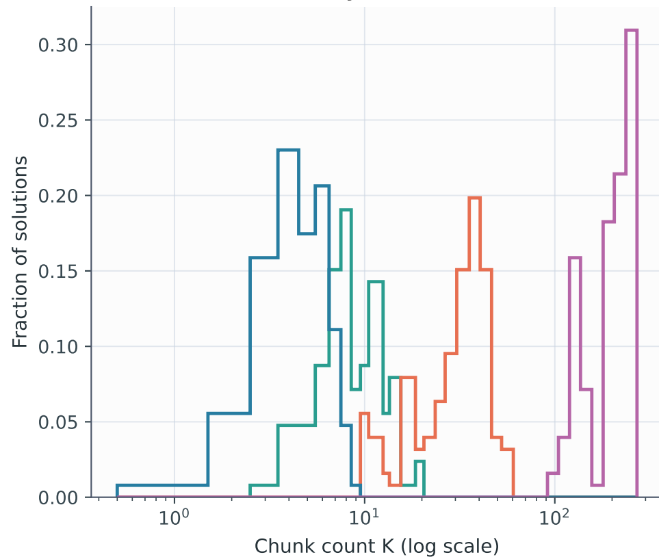
Locally clustered
