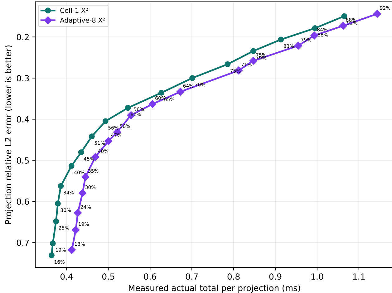
Global importance lower bound (labels are resulting R)
