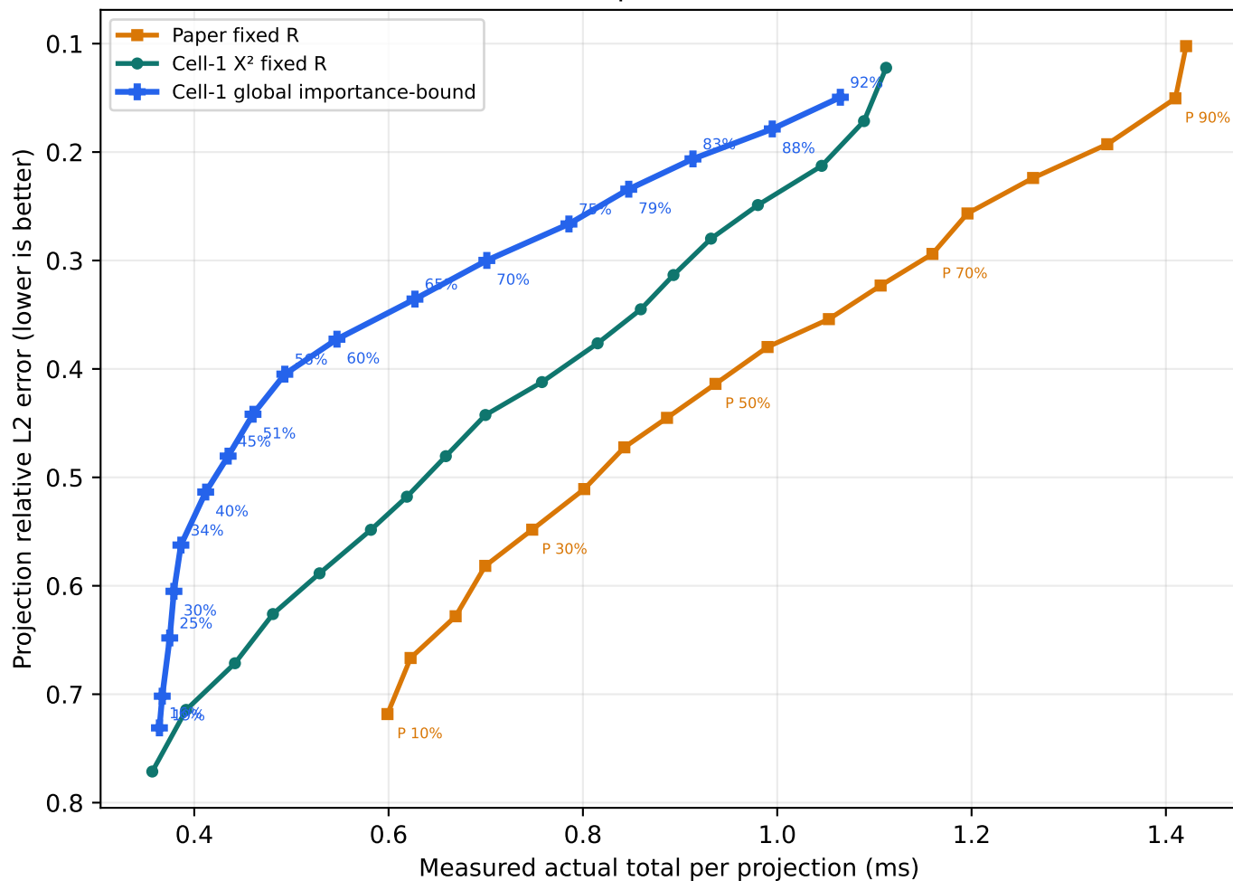
Measurable importance lower bound
