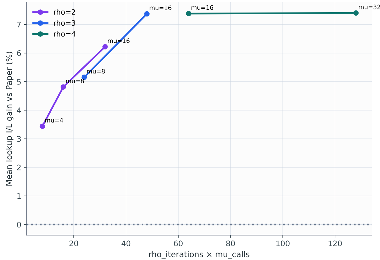
CUDA round trip: quality vs maximum DP calls
