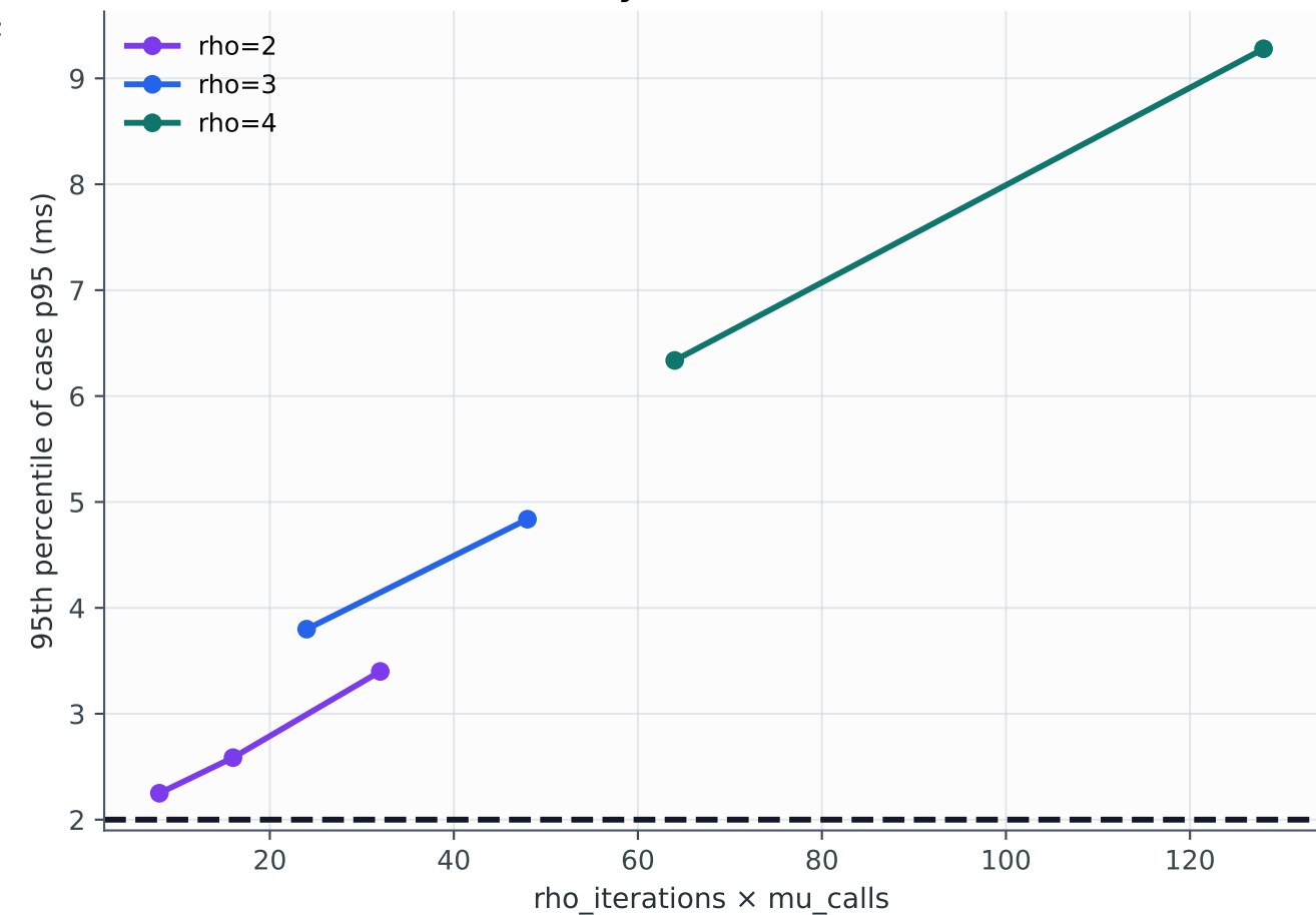
CUDA round trip: latency vs maximum DP calls
