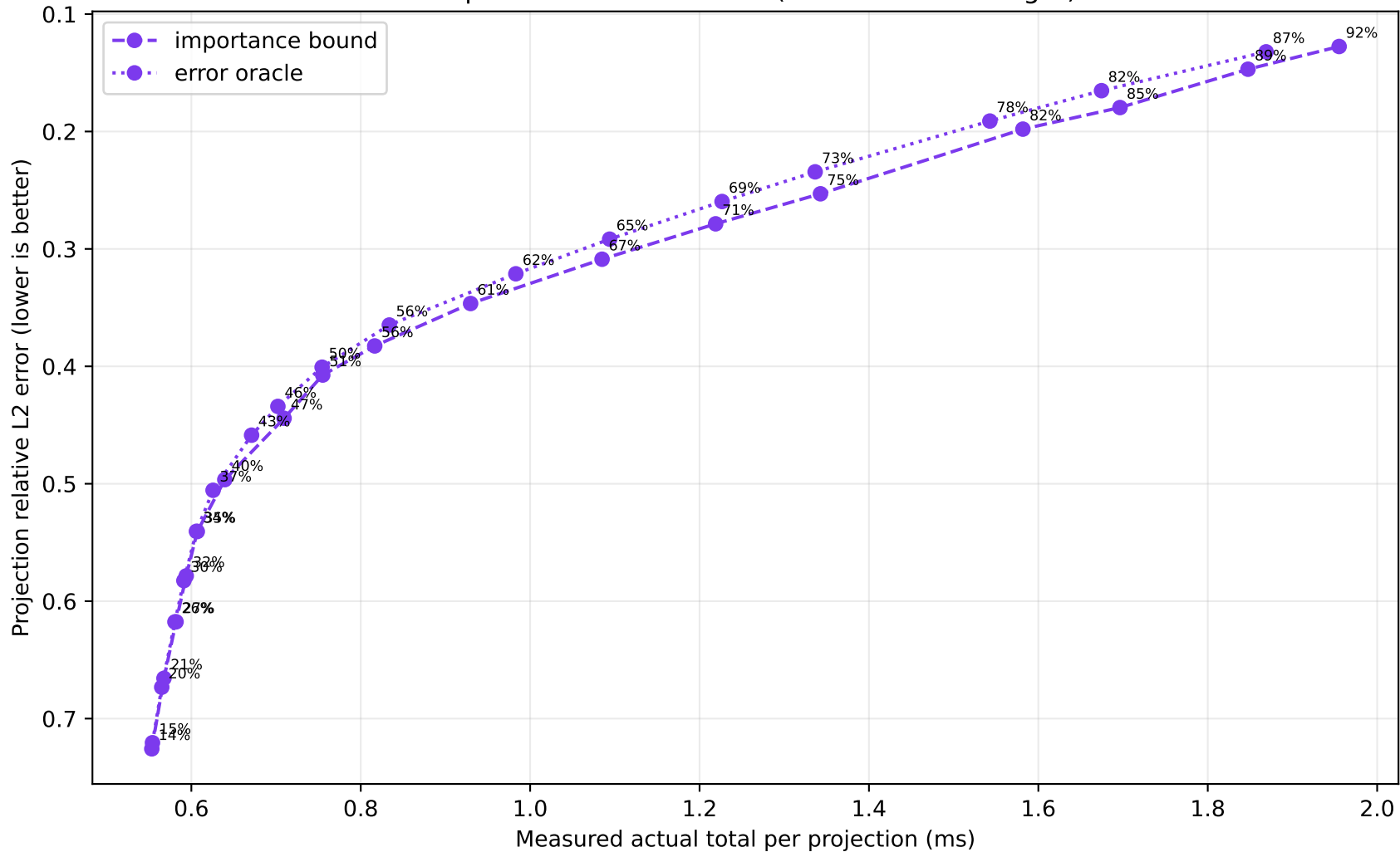
Adaptive-8 without fixed R (labels are resulting R)
