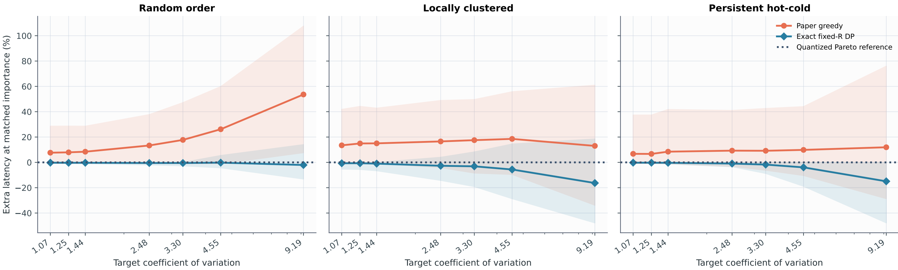
Latency relative to Quantized Pareto at each fixed-R method's achieved importance
