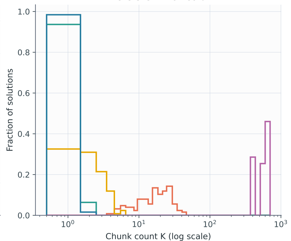
Persistent hot-cold
