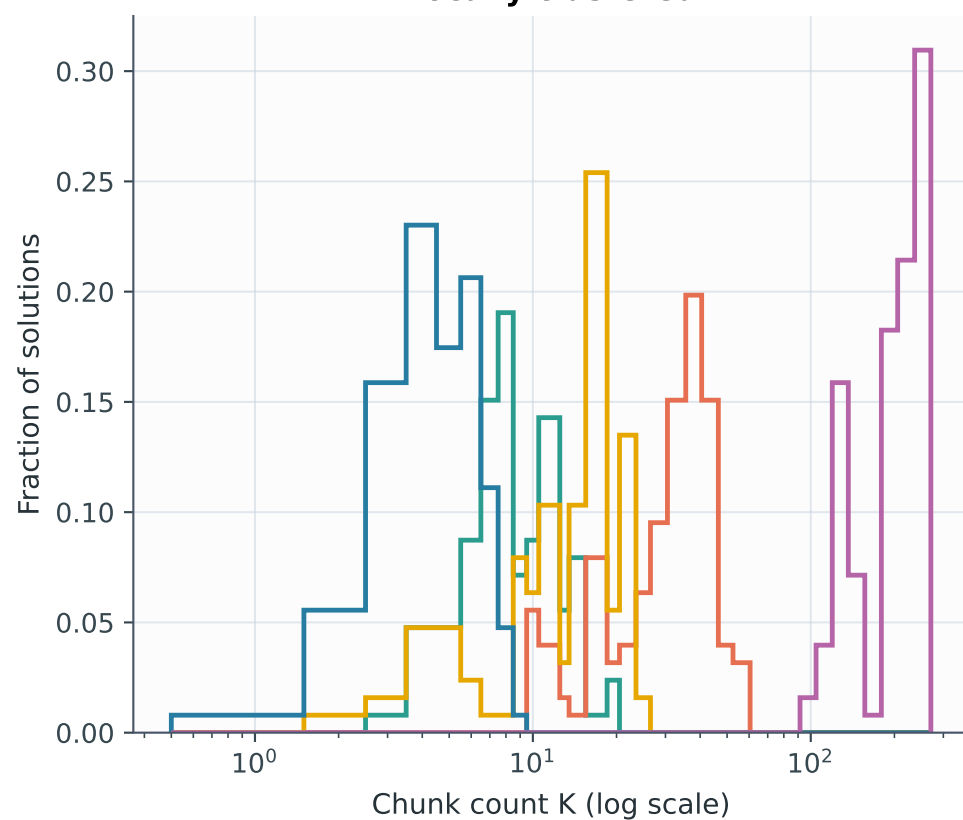
Locally clustered
