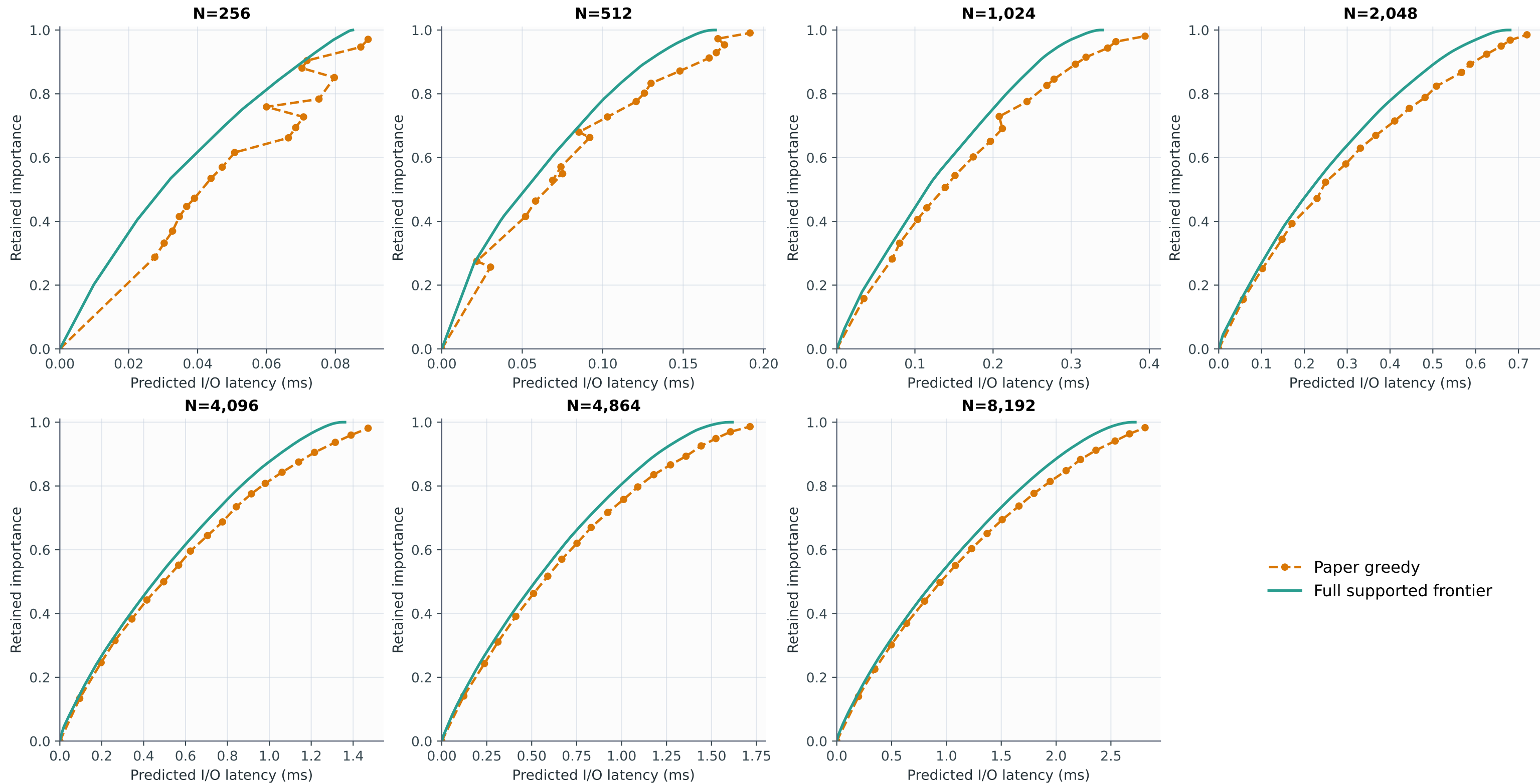
Lookup example frontiers (trial 0, random order)
