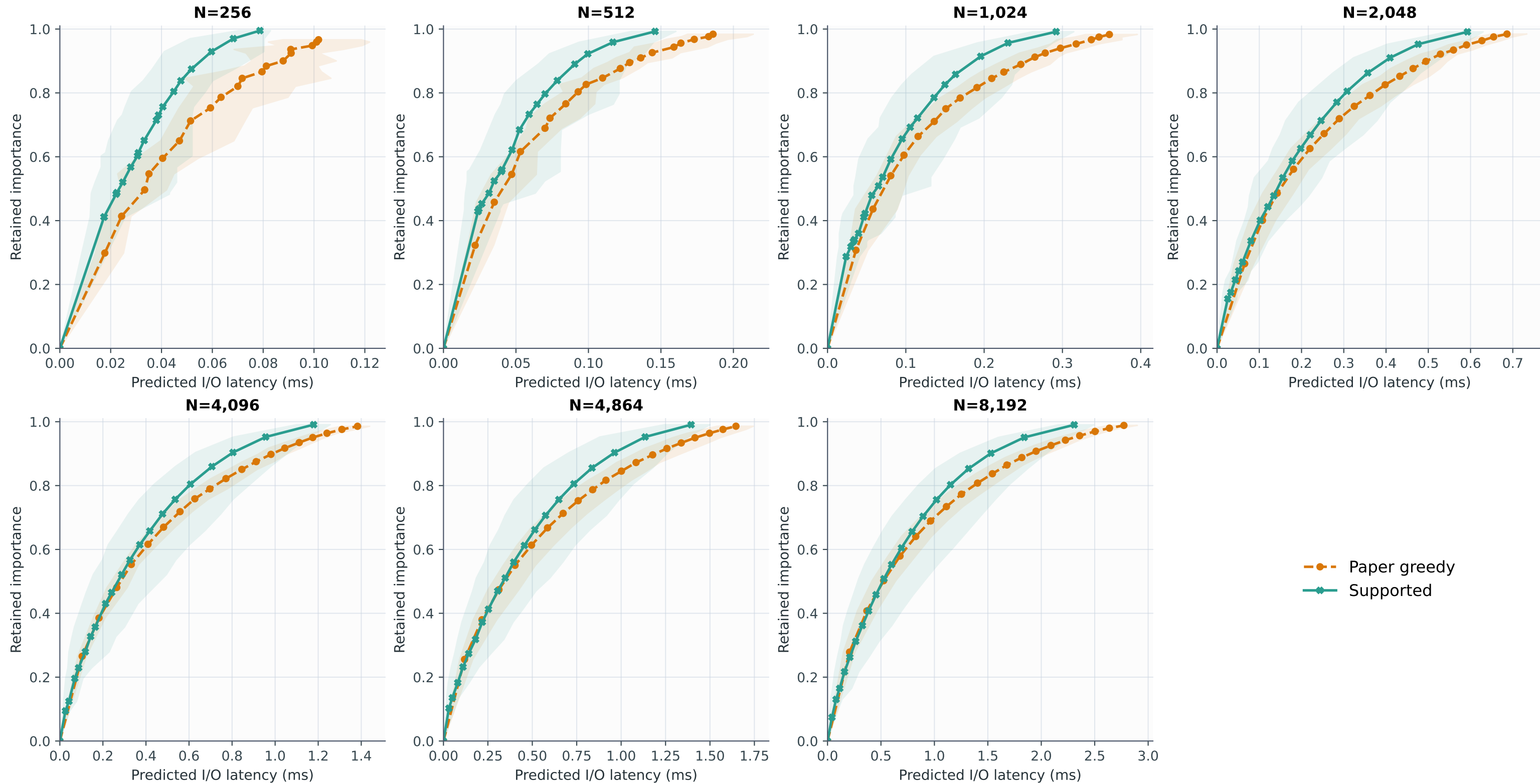
Two Line importance-latency curves
