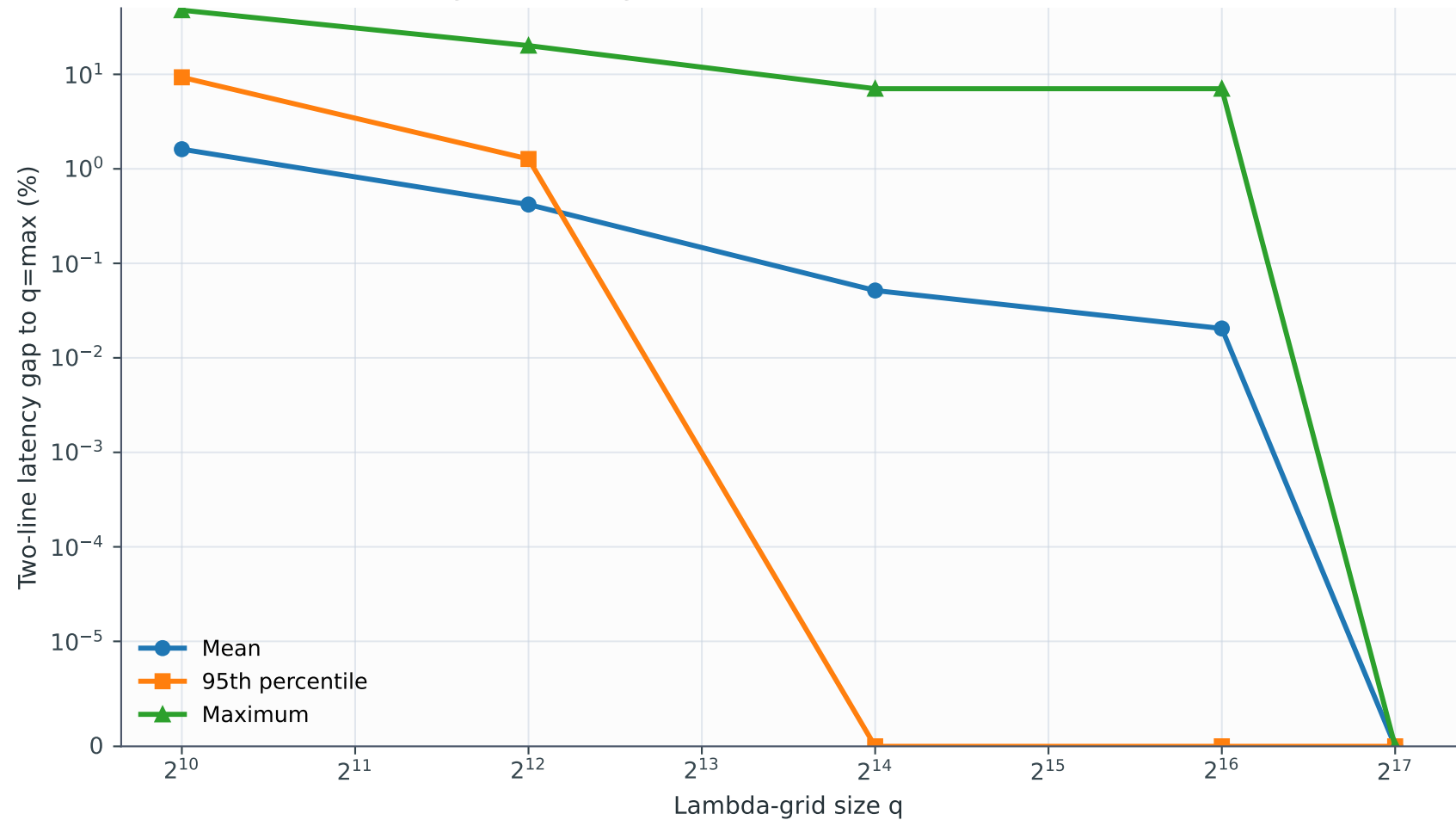
Dense-grid convergence (not an exact-optimum certificate)
