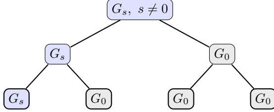
FIGURE 1. Two generations of lifts (Proposition 3.3). A shift-nonzero obstruction (blue) splits into one shift-nonzero and one shift-zero child; a shift-zero obstruction (grey) splits into two shift-zero children. Shift-zero is therefore absorbing under lifting: it never produces a shift-nonzero residue. The single persisting shift-nonzero line, shedding one shift-zero child per level, is the combinatorial engine behind the strict lift balance of Corollary 6.4.
