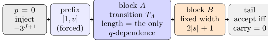
FIGURE 2. Block factorisation of the carry automaton of Lemma 6.11. Only the length of block A depends on q ; the transition T_A does not. As T_A^m(R_0) is eventually periodic, a finite computation over one preperiod and one period decides the stratum for all q . The fixed-point data (preperiods, periods, reachable-state counts) per stratum are tabulated in Appendix A.
