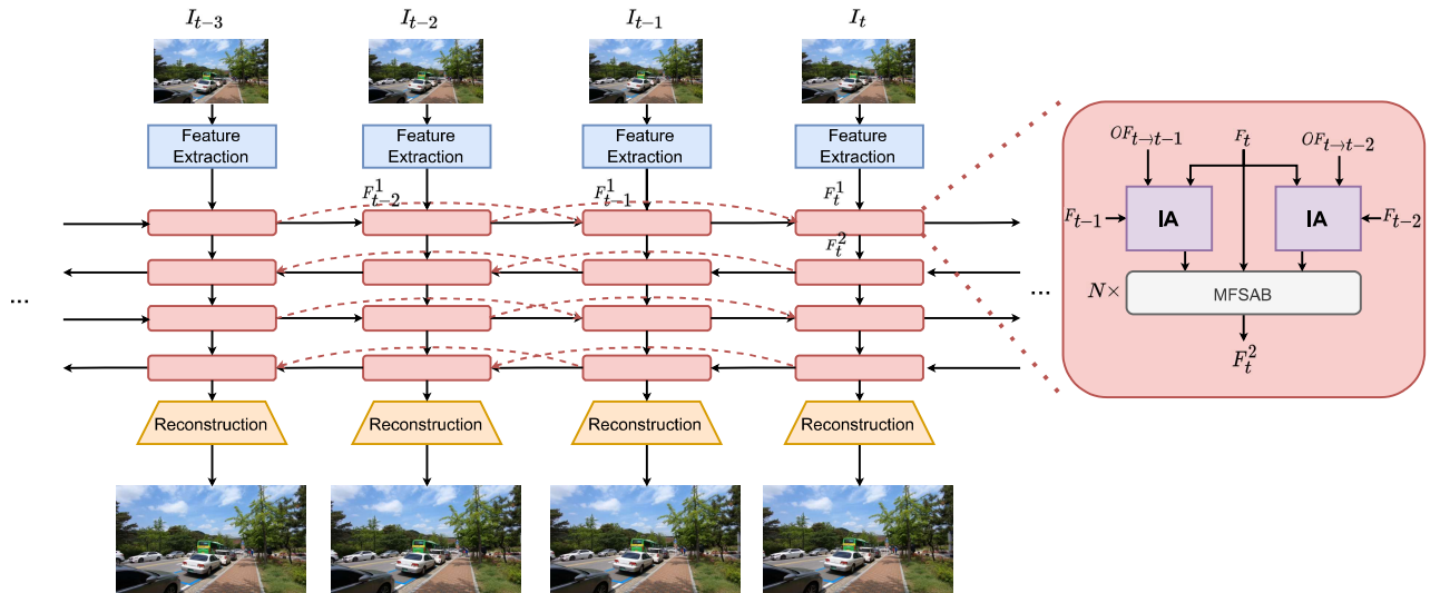
Figure 2. Network Structure for IA-RT.
