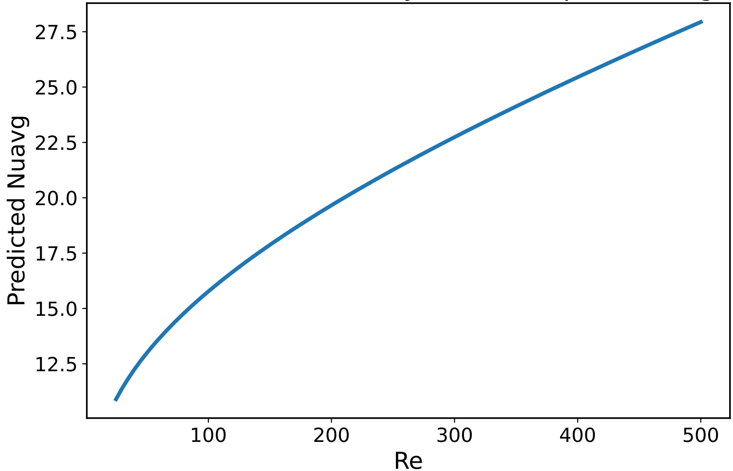
Selected-correlation Reynolds sweep for Nuavg
