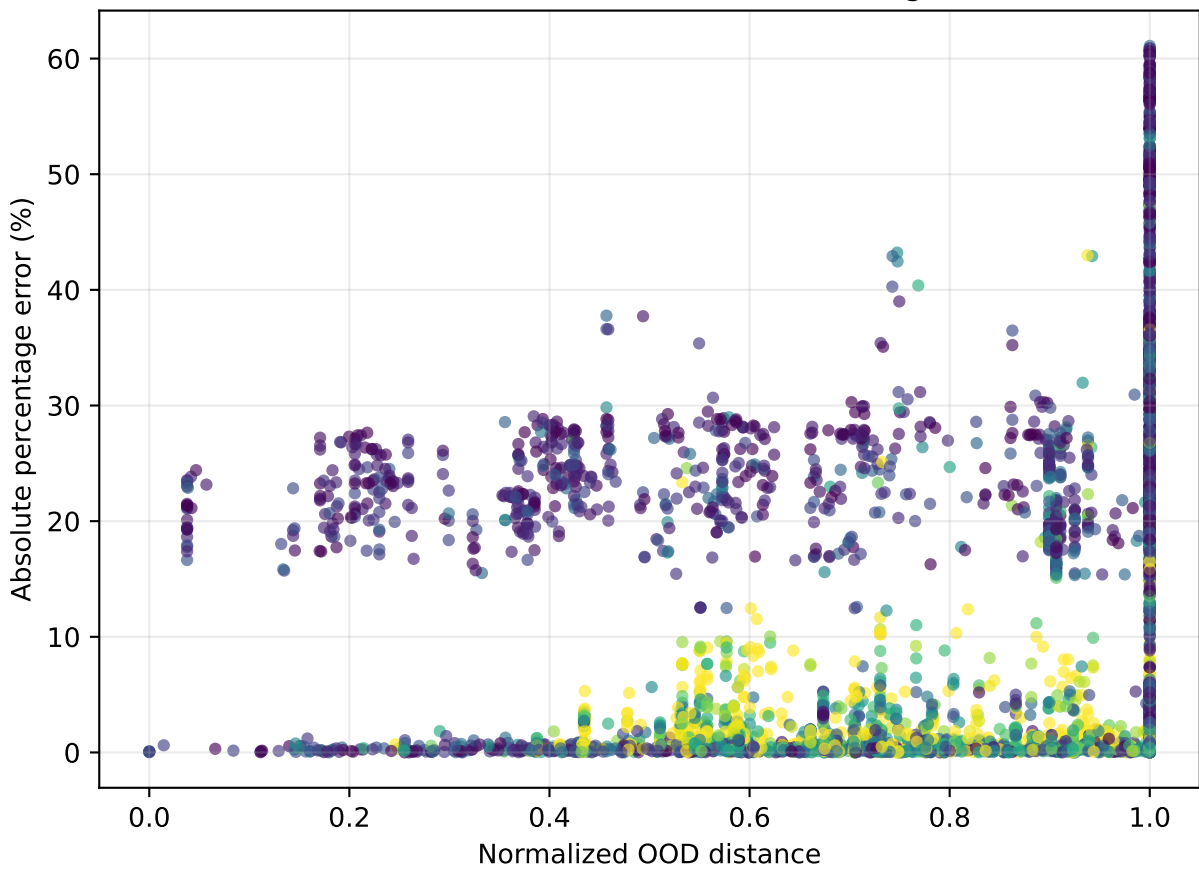
Error versus OOD distance: Nuavg
