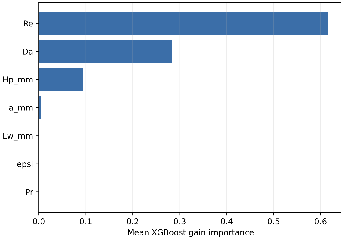
Feature importance: DelP_Pa
